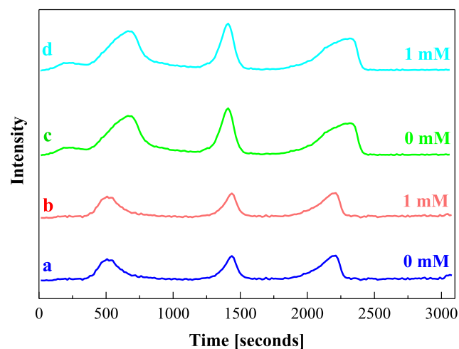
Fig. 5. Gram-Schmidt curves a) Calcium oxalate (CaOx) crystals synthesized in aqueous solution without hyaluronic acid (HA). b) CaOx crystals synthesized in aqueous solution with 1 mM HA. c) CaOx crystals synthesized in artificial urine without HA. d) CaOx crystals synthesized in artificial urine with 1 mM HA.
