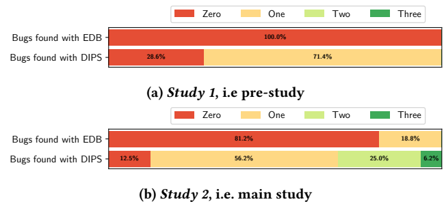
Figure 8: Number of bugs found by users participating in both studies, categorized per debugger system.
