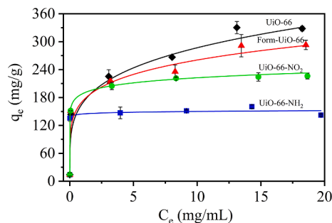
Fig. 3. Mo adsorption isotherms of UiO-66 (black), UiO-66-NH 2 (blue), Form-UiO-66 (red) and UiO-66-NO 2 (green) at \text{pH} 3.
