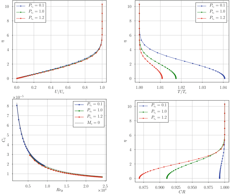
Fig. 5. Results for MM in ideal and NICFD conditions at M_e = 2 . Top: dimensionless velocity and temperature distribution. Bottom: dissipation coefficient and Chapman-Rubinsin parameter within the boundary layer.
