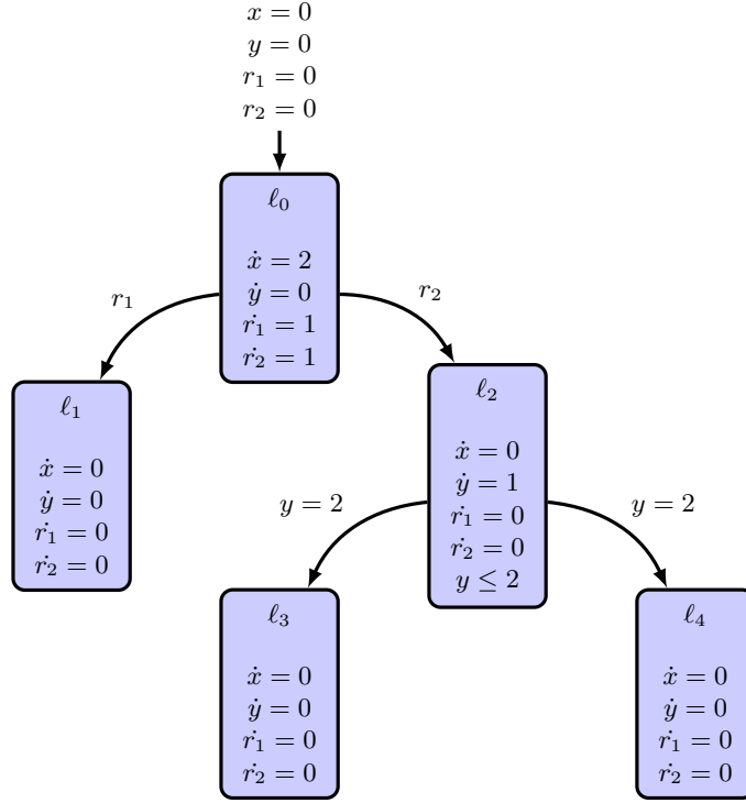
Figure 4: Case B modelled as a rectangular automaton with random clocks (RAR).
