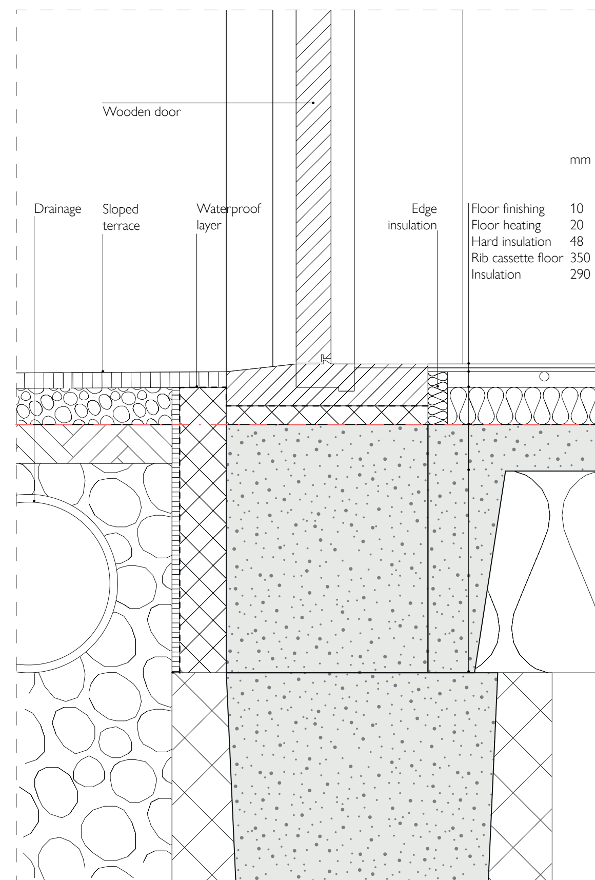
Detail 2
