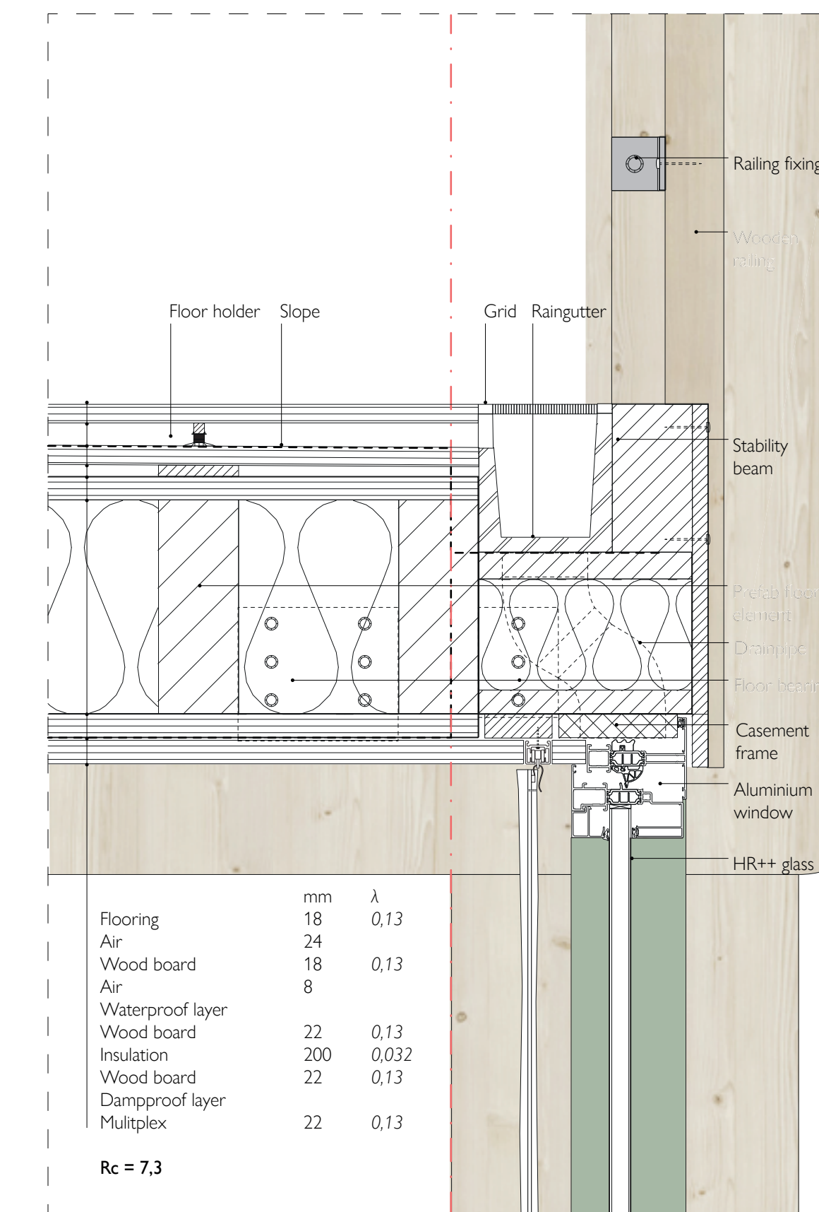
Detail 5
