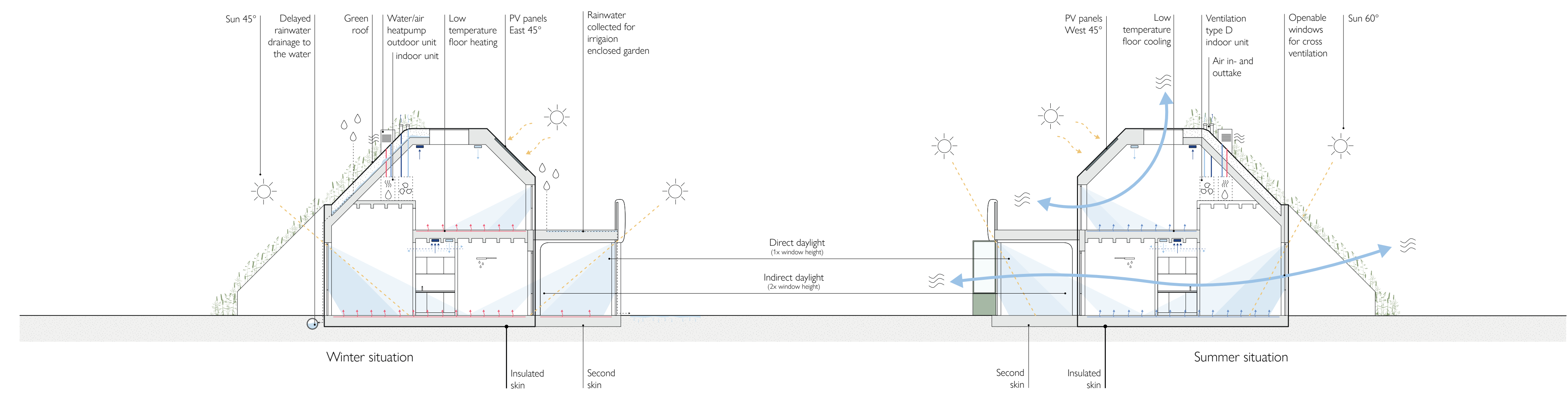
Climate section | 1 : 200
