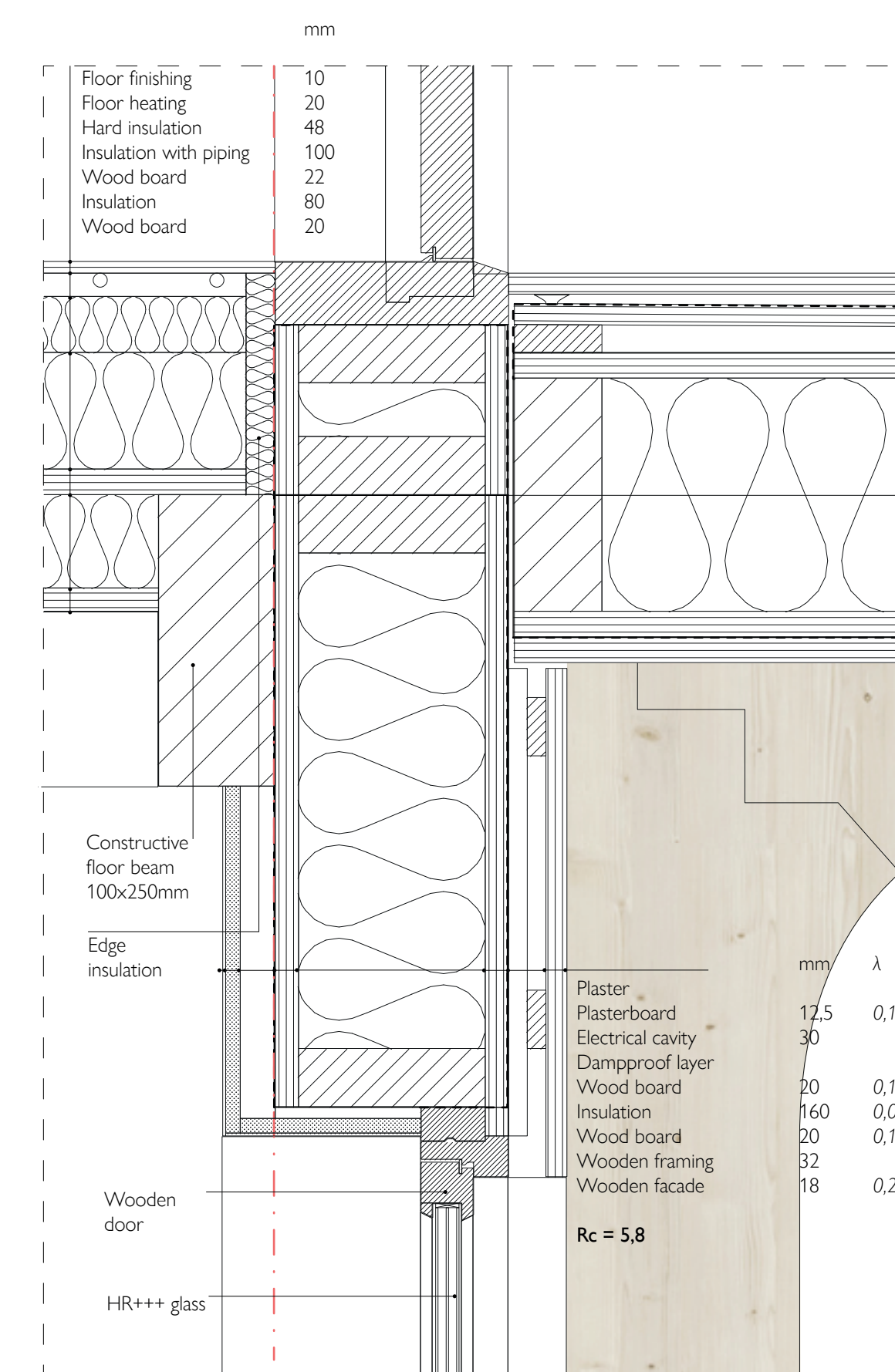
Detail 4
