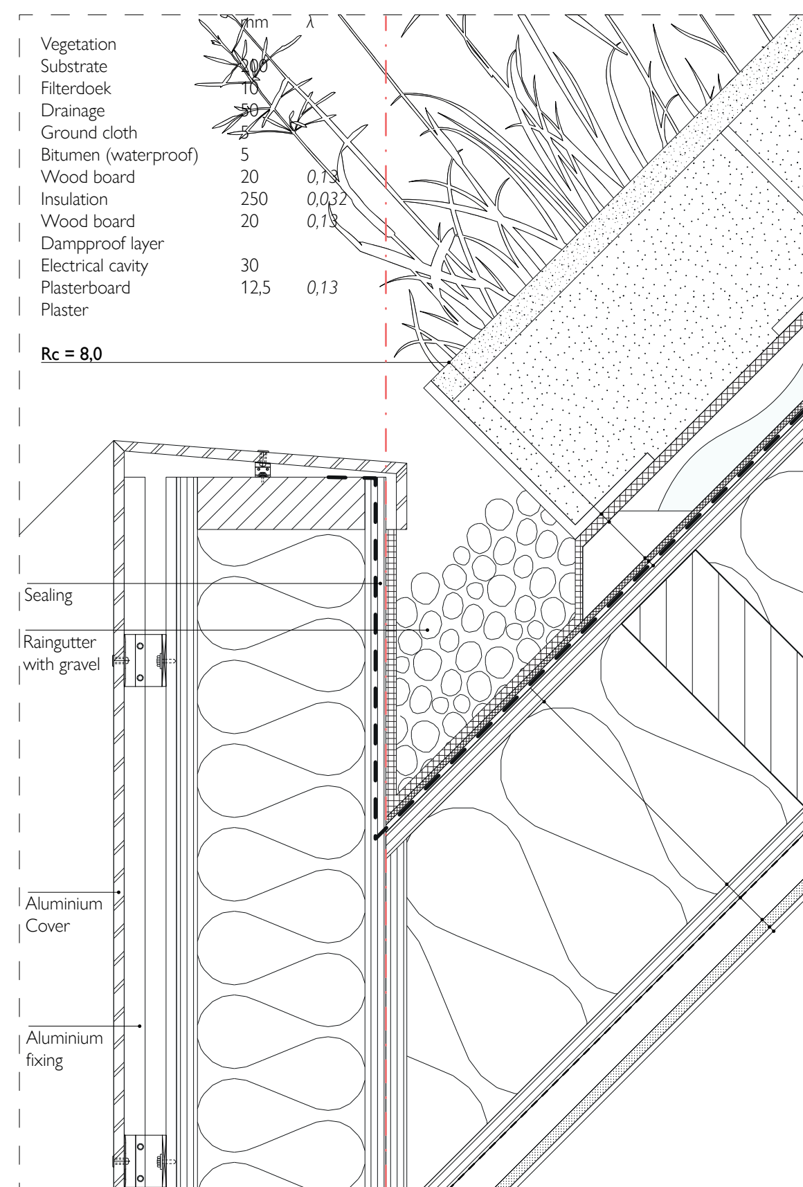
Detail 1
