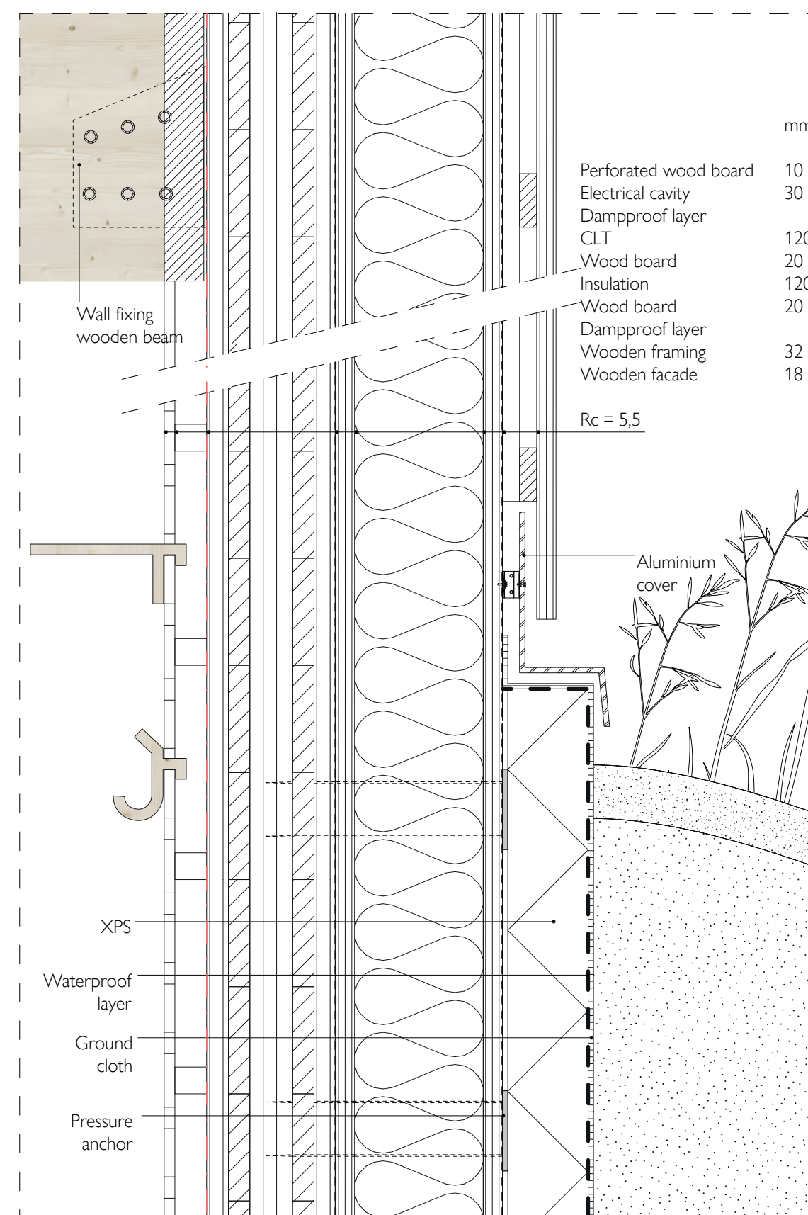
Detail 3.1 & 3.2
