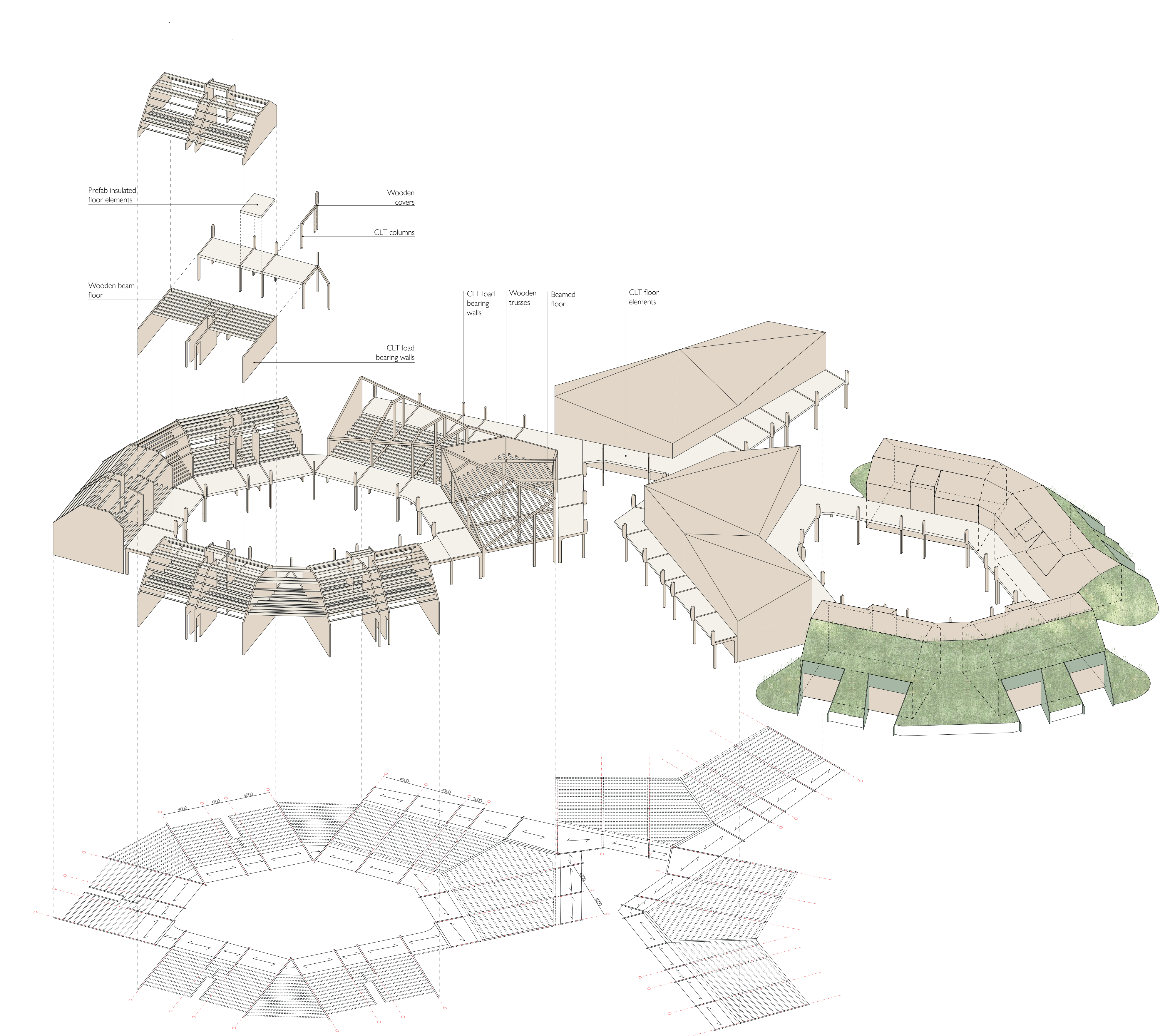
Axonometric building structure | 1 : 200
