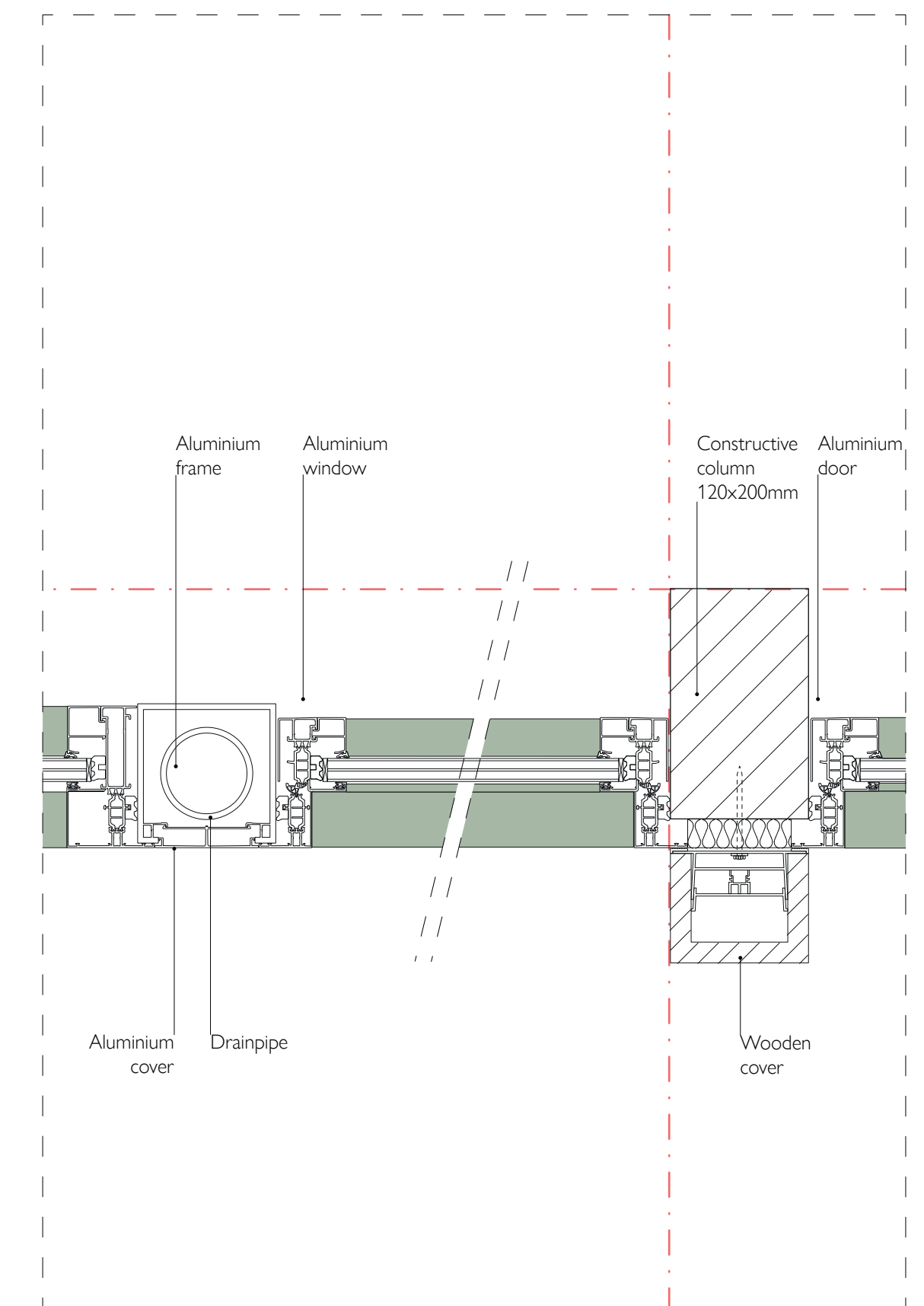
Detail 6.1 & 6.2
