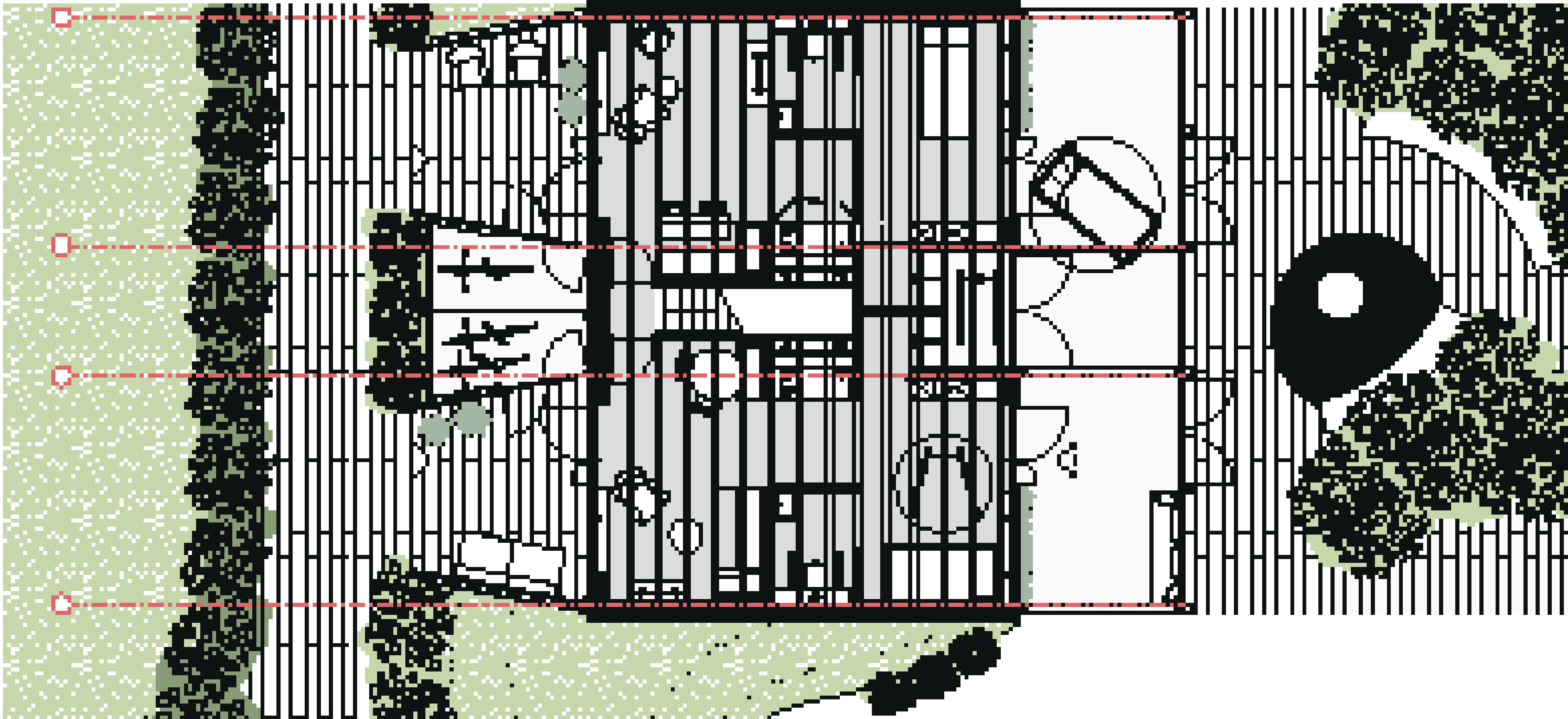
Floor plan residents room (ground floor) | possible furnishing | 1 : 50
