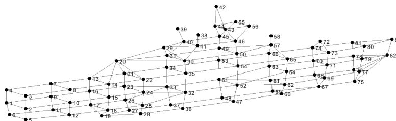
Figure 2: Layout of the notional OPV used for the test case. Each node represents the geometric centre a compartment. Each edge denotes a physical adjacency between compartments, i.e. the compartments are located on both sides of the same deck or bulkhead.
