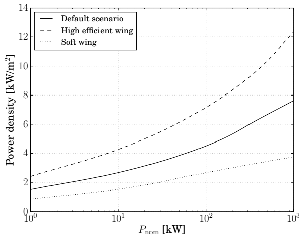
Figure 3. Power per square meter of wing area. As comparison: Average silicon solar modules achieve currently (2015) a power density of just about 0.15 kW per m 2 .
