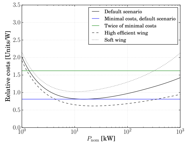
Figure 9. Costs per W nominal generator power.
