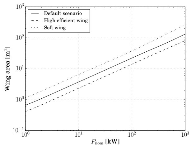
Figure 4. Wing area of an optimized airborne wind energy system for different power ratings. A good approximation for the default scenario is the following equation: A = 0.62 p_{\text{nom}}^{0.77} . The resulting error is \leq 5\% .
