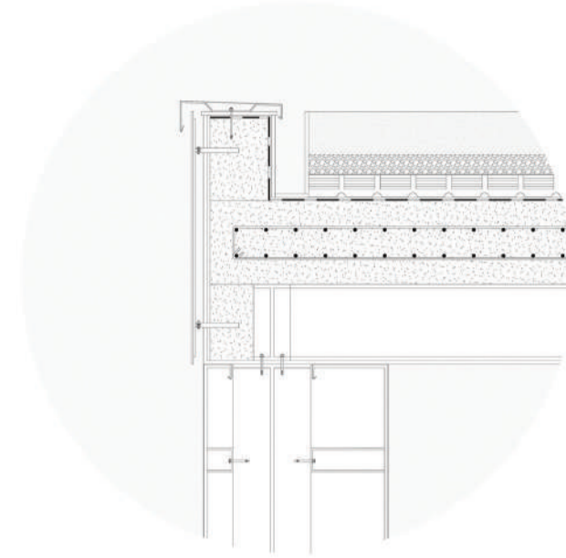
DETAILED ROOF
