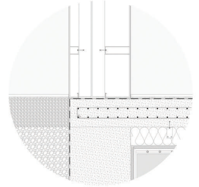
DETAILED FOUNDATION
