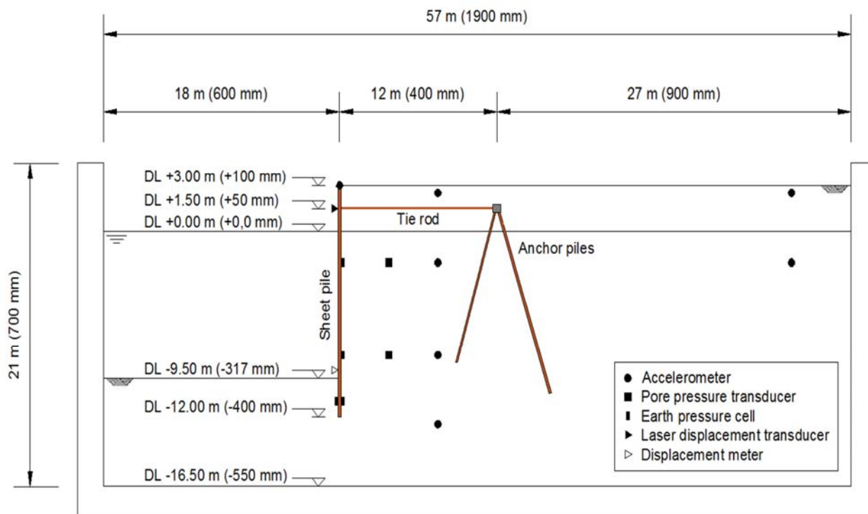
Fig. 3 Reference case test model for centrifugal shake-table experiments, adapted from [10]
