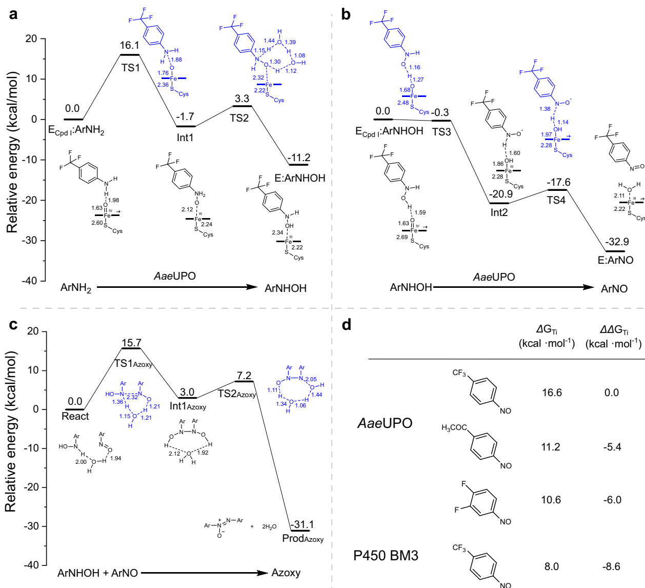
Fig. 5 | Mechanistic study of the AaeUPO-catalyzed azoxy compound synthesis from aniline. The energy profiles for the catalytic oxidation of ArNH 2 to ArNHOH (a), the subsequent oxidation of ArNHOH to ArNO (b), the formation of
