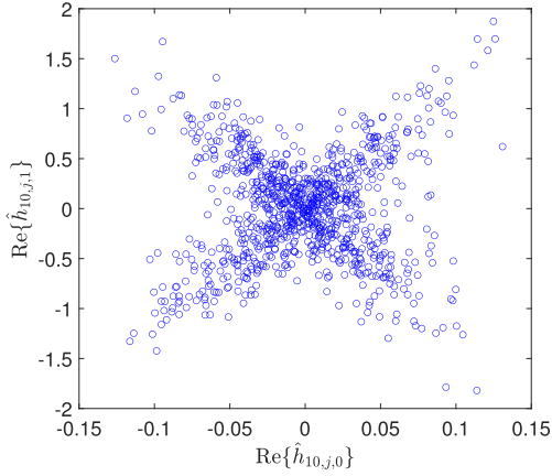
Fig. 6. Scatter plot of \Re\{\hat{h}_{10,j,1}\} and \Re\{\hat{h}_{10,j,0}\} when device k = 10 is active, K_u = 1536 , N_c = 512 , P_a = 0.01 , and \text{SNR} = 16 dB.
