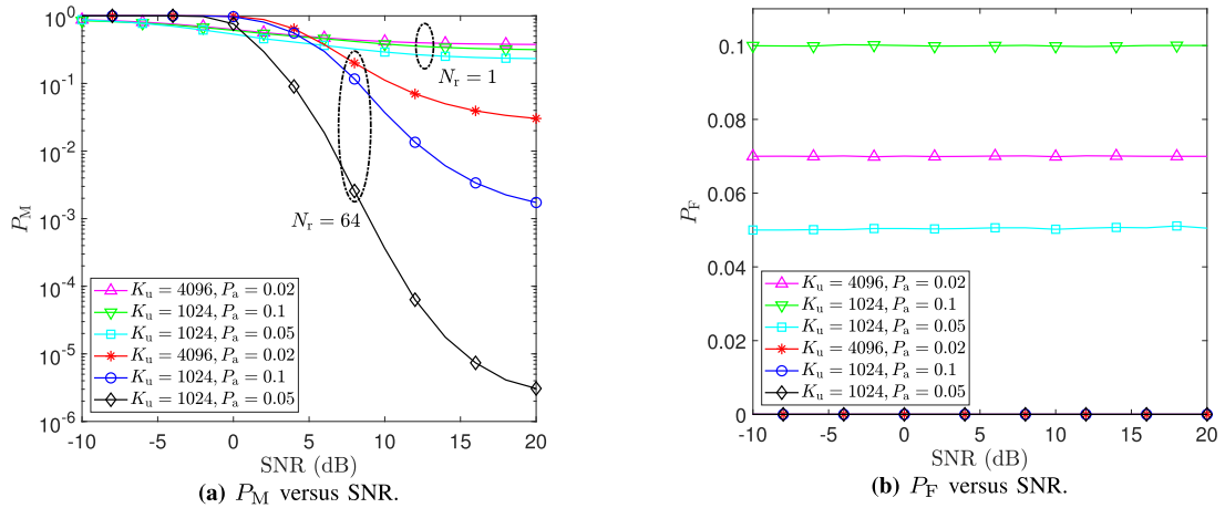
Fig. 9. Performance of the proposed \ell_2 -norm SSR IoT DI algorithm for P_f^{(k)} \in \{0.05, 0.07, 0.1\} , K_u \in \{1024, 4096\} , L = 1 , and N_r = \{1, 64\} with the majority hard decision combining.
