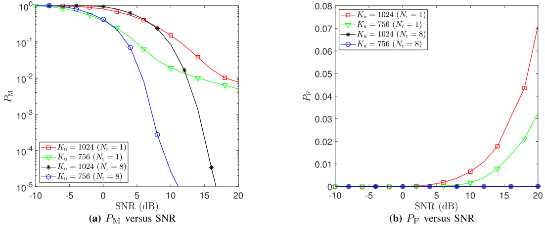
Fig. 12. The system miss identification rate, P_M , and false alarm rate, P_F , of the proposed BIC \ell_1 - \ell_2 mixed-norm SSSR IoT DI algorithm (Algorithm 2) versus SNR for random activity rate P_a \in [0, 0.06] and L = 21 with the majority rule hard decision combining.
