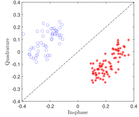
Fig. 7. Separated symbols by the proposed 2-MC-MUD algorithm for an active IoT device at 10 dB SNR, K_u = 768 , and N_c = 512 .
