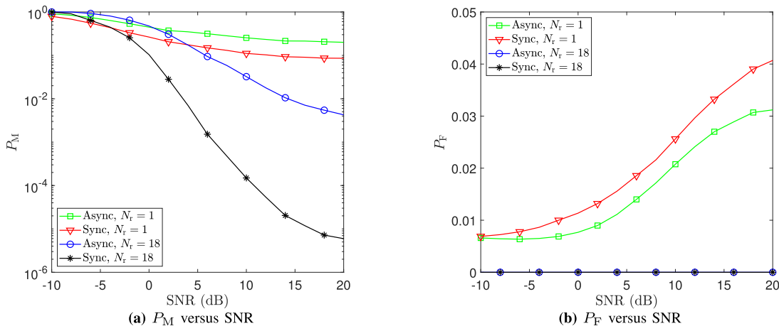
Fig. 11. Effect of uncertainty in delay \tau_k , k \in \mathcal{X}_u , on the performance of the proposed \ell_2 -norm SSR IoT DI algorithm for P_a = 0.05 , K_u = 1024 , N_r = \{1, 18\} , L = 21 , and P_f^{(k)} = 0.06 .
