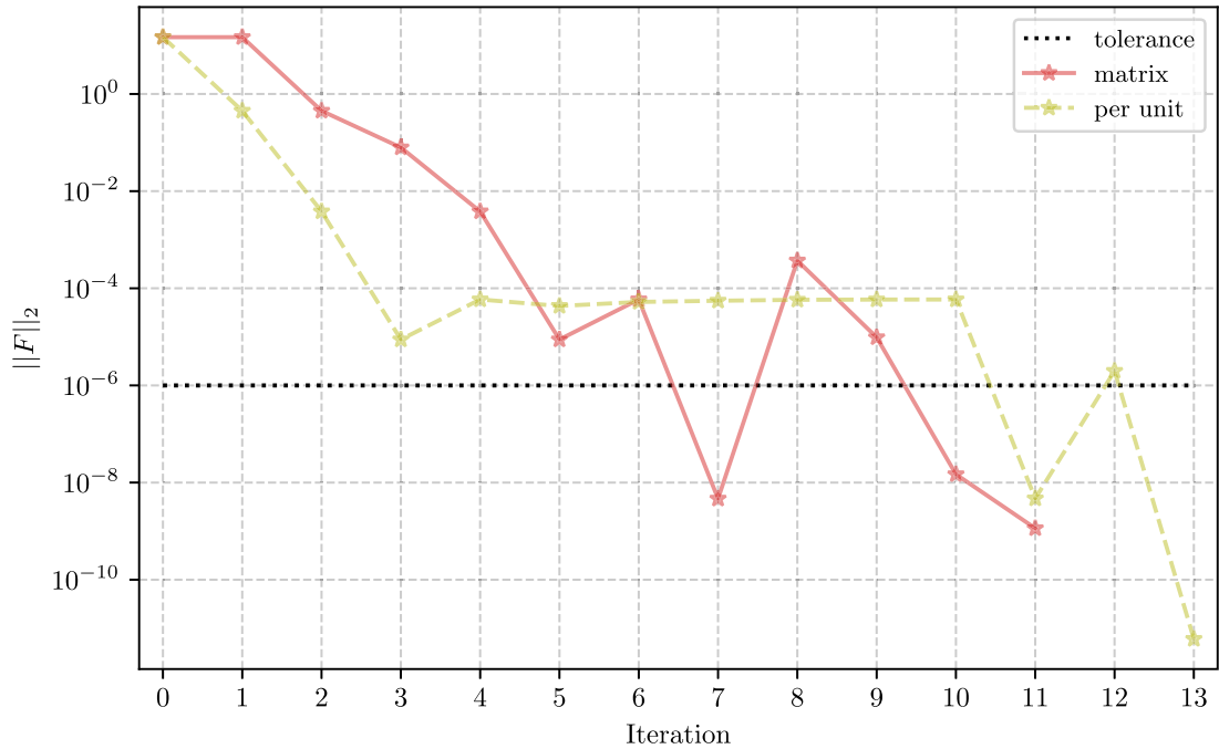
Fig. 5. Error of scaled LF equations \|F\|_2 at every iteration of the optimizer for the OF problem of the base network, without bounds on q_k , m_{i,j} , and |S_k|^2 , nodal formulation in gas, and terminal link flow formulation in heat, using formulation I and SLSQP. Comparison of matrix scaling and per unit scaling.
