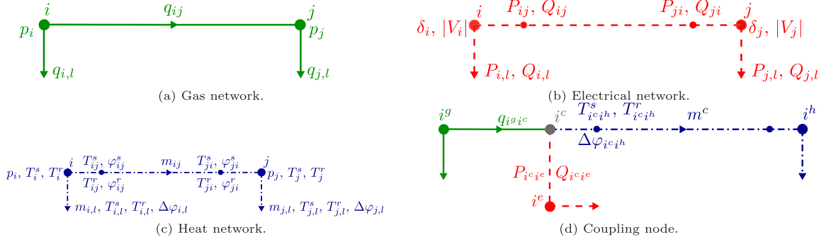
Fig. 1. Quantities of interest for load flow simulation of energy systems, and the network elements they are associated with. Arrows on links and terminal links show defined direction of flow.
