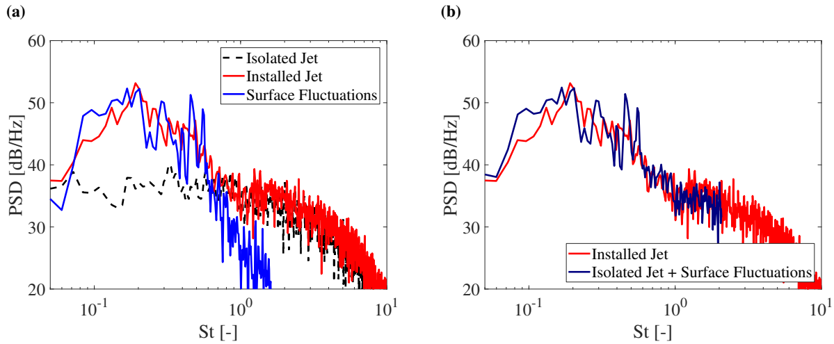
Fig. 15 Far-field spectra of the pressure fluctuations on the flat plate, compared to results the from the permeable FWH surface (isolated and installed jets)
