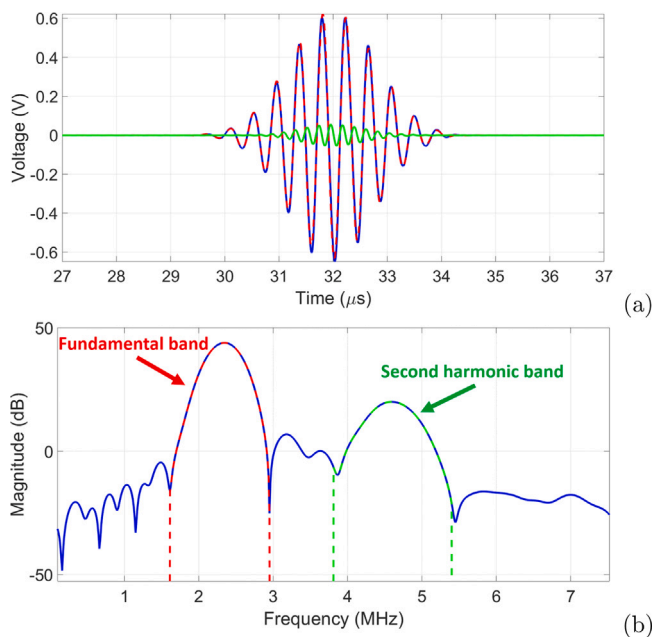
Fig. 4. (a) A measured nonlinear time signal during flow measurements (blue), as well as its fundamental (red) and second harmonic (green) components. (b) Magnitude of the Fast Fourier Transform (FFT) applied on the time signal shown in (a).
