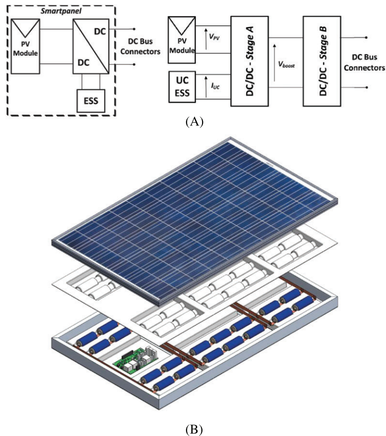
FIGURE 9 A, System components (left), power conversion stages (right); B, complete integrated system. Reproduced with permission with Dede et al. 139 Copyright 2016, IEEE [Colour figure can be viewed at wileyonlinelibrary.com ]
