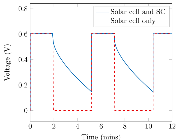
FIGURE 1 Response of a single solar cell and a solar cell coupled with a supercapacitor during intermittent illumination. If light is on, the voltage of a single solar cell is around 0.6, but when light is off, the voltage decreases to 0. In cases where an appropriate SC is used, the system voltage does not decrease to zero intermediately in the absence of light. This figure is based on Ouyang et al, 16 where the illumination period was 2 min followed by a 3-min discharging process at a constant discharging current density of 40 \mu\text{A cm}^{-2} [Colour figure can be viewed at wileyonlinelibrary.com ]
