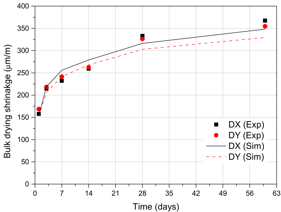
Fig. 8. Bulk drying shrinkage of concrete slice’s surface layer in X and Y directions obtained by 3D-DIC and lattice fracture model. DX = Direction of X-axis, DY = Direction of Y-axis, Exp = Experiment, Sim = Simulation.
