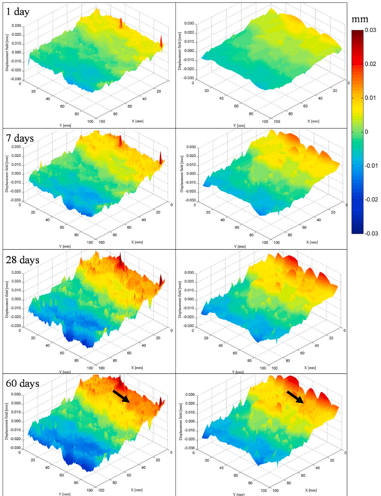
Fig. 5. Displacement fields in direction of X-axis: 3D-DIC measurement (left) versus lattice fracture simulation (right).
