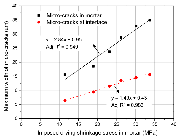
(b) Maximum width of micro-cracks.
