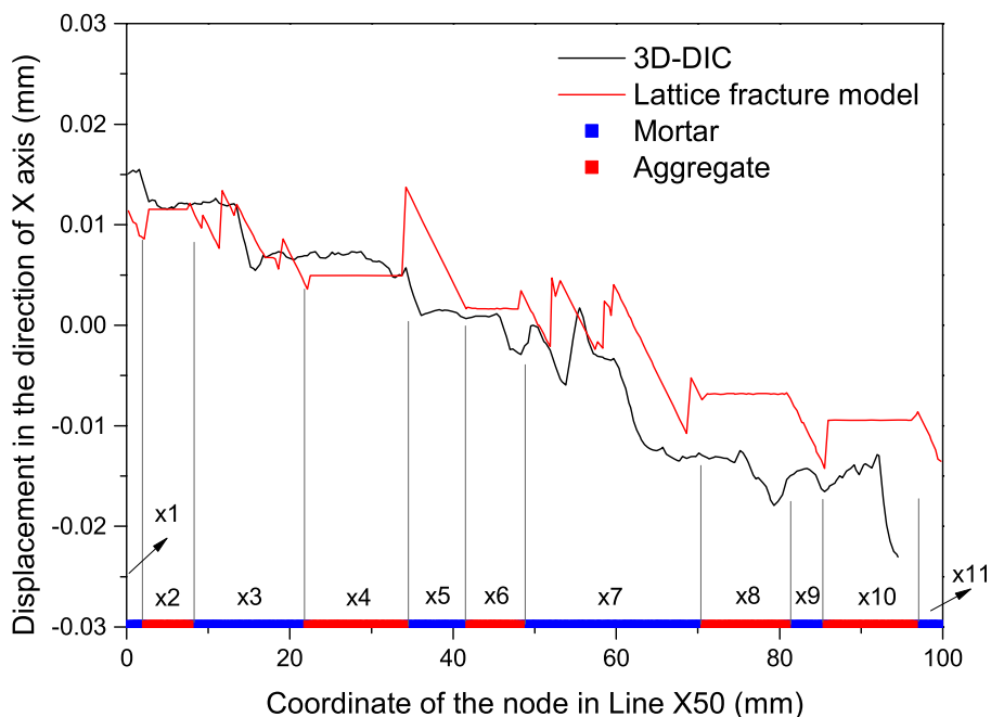
(a) Displacement field in line X50.
