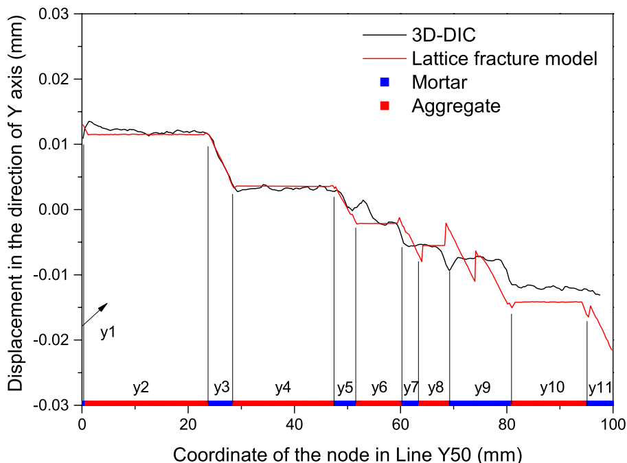
(b) Displacement field in line Y50.
