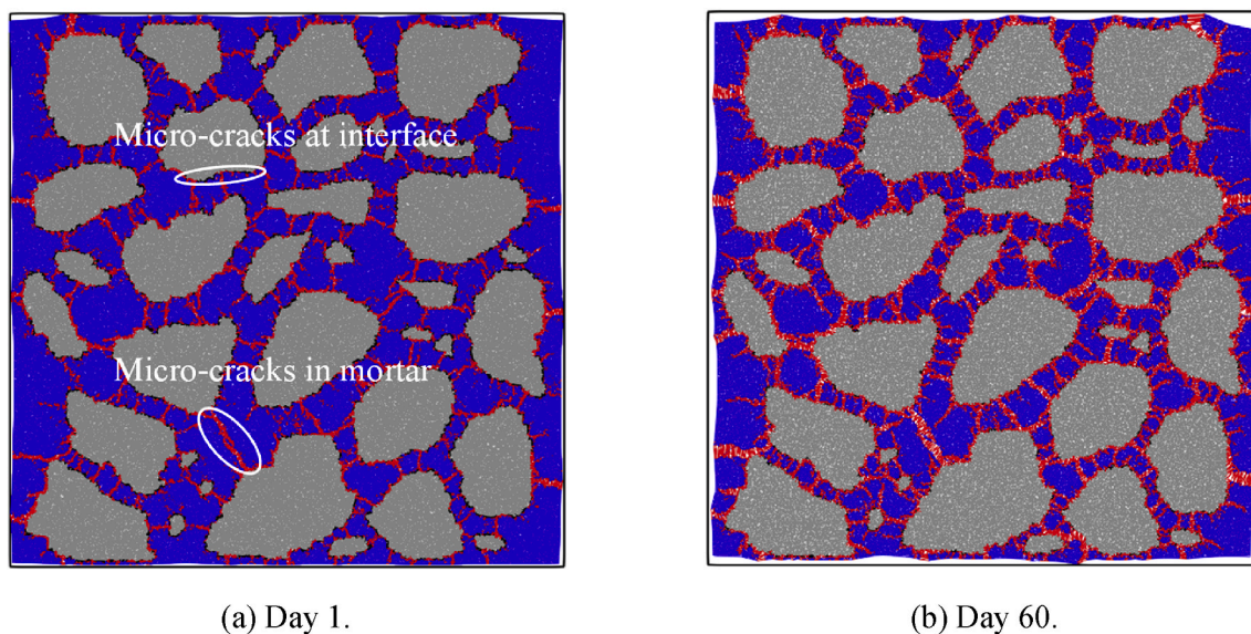
Fig. 9. Simulated drying-induced micro-crack propagation in surface layer of concrete slice that dried at day 1 and day 60. Note: the deformations are magnified 80 times for visualization purposes.
