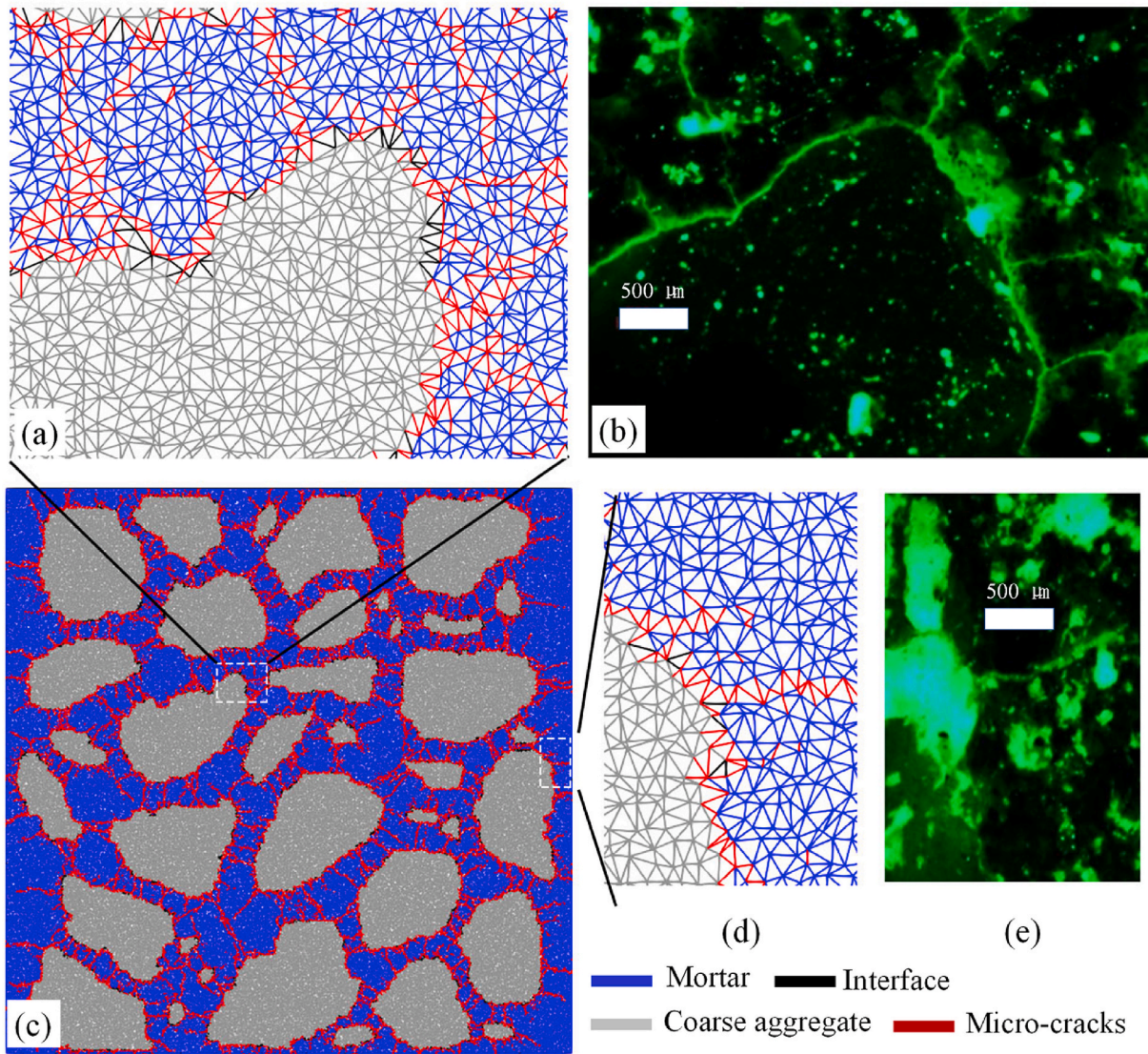
Fig. 10. Micro-crack patterns obtained by lattice fracture simulation and fluorescent resin measurement for concrete that dried for 60 days: (a), (c) and (d) are patterns obtained by the lattice fracture model; (b) and (e) are the patterns obtained by the fluorescent resin measurement. Note: the deformation is not magnified.
