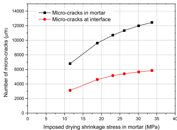
(a) Number of micro-cracks.
