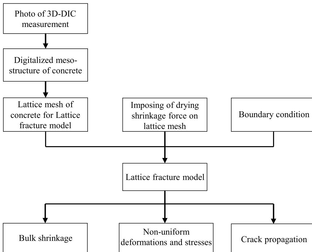
Fig. 1. Outline of simulation of drying-induced non-uniform deformations, stresses, and crack propagation in concrete using GLAK.
