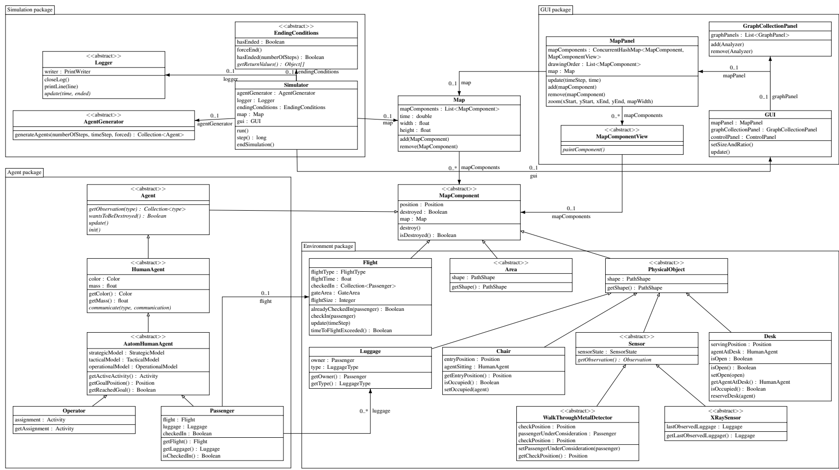
Figure 7: The UML class diagram of AATOM.
