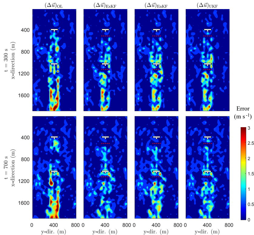
Figure 4. Comparison of absolute values of the estimation errors (in long. flow fields) for state-only estimation with the ExKF, EnKF and UKF at t = 300 s and t = 700 s, with (\Delta \mathbf{u}) = |\mathbf{u} - \mathbf{u}_{\text{SOWFA}}| . The model and KF settings are depicted in Tables 1, 2, and 3. Wind is coming in from the top, flowing towards the bottom. The measured states are depicted by red dots in the flow, not to be confused with estimation error. The KFs consistently improve the instantaneous flow field estimations, noticeably nearby the measurements.
