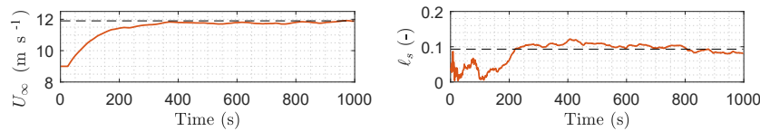
Figure 7. Convergence of \ell_s and U_{\infty} using the EnKF. Dashed lines are the grid-searched optimal constant values for the open-loop simulation. With power measurements only, the EnKF is able to estimate these parameters successfully in addition to the model states.
