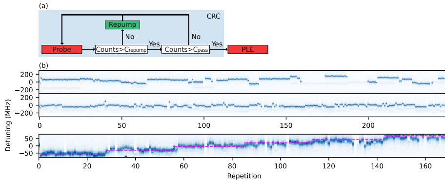
Fig. 2. (a) CRC pulse sequence protocol. (b) CRC preceded PLE scans, for a low (high) C_{\text{pass}} in the top (middle) panel. Bottom panel: CRC preceded PLE scans with changing frequency set point.
