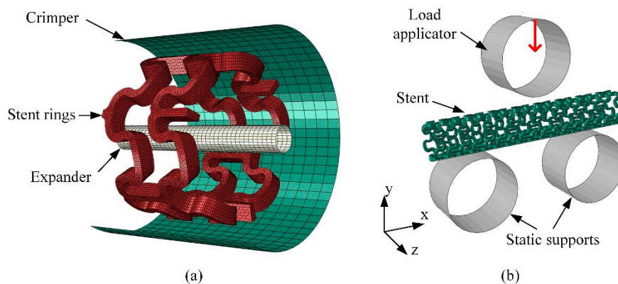
Figure 4. 3-D finite element (FE) models for (a) deformation tests and (b) three-point bending tests.
