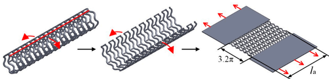
Figure 3. Planar specimen with a chosen stent design pattern for the stretching tests.
