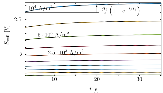
Fig. 4. The measured cell voltage increase for c = 6 M (solid lines) can be fitted well with Eq. (8) (dashed lines — approximately overlapping). The fitting parameters l_t \approx 1.1 mm and t_b \approx 10 s for the highest current density both only very slightly increase with decreasing current density, see Appendix A.
