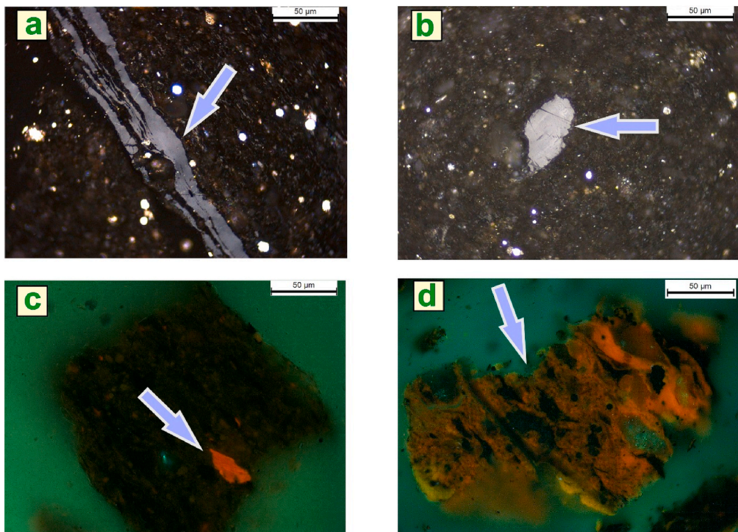
Fig. 9. Fragments of graptolites and alginite particles (Jantar Formation). (a,b) Longitudinal and perpendicular cross sections of graptolites, (c, d) alginite exhibits fluorescence under UV light (colour points to thermal maturity between oil and wet gas windows). (For interpretation of the references to colour in this figure legend, the reader is referred to the Web version of this article.)
