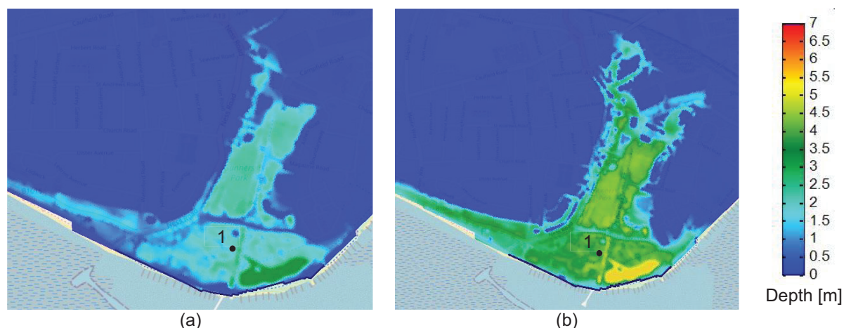
Figure 4. Results of Delft3D numerical simulations for the scenario without additional measures: (a) without SLR; (b) with SLR of +60cm by 2100.
