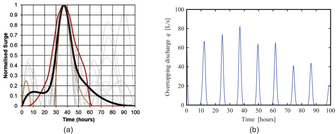
Figure 3. (a) Synthetic surge at Sheerness (UK). (b) Overtopping discharge over the crest length of 1,000 m and a storm duration of 100 hours.
