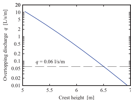
Figure 7. Relationship between overtopping discharge and crest height. Data shows that for an overtopping discharge q < 0.06 L/s/m, a crest height of \sim 6.5 m is necessary.
