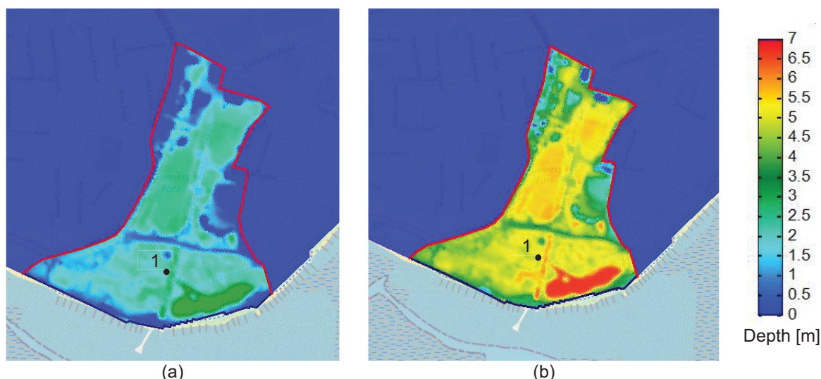
Figure 5. Results of Delft3D FM numerical simulations for the scenarios with additional internal barriers to contain the flooded water in the Gunners Park area: (a) without SLR; (b) with SLR of +60cm by 2100.
