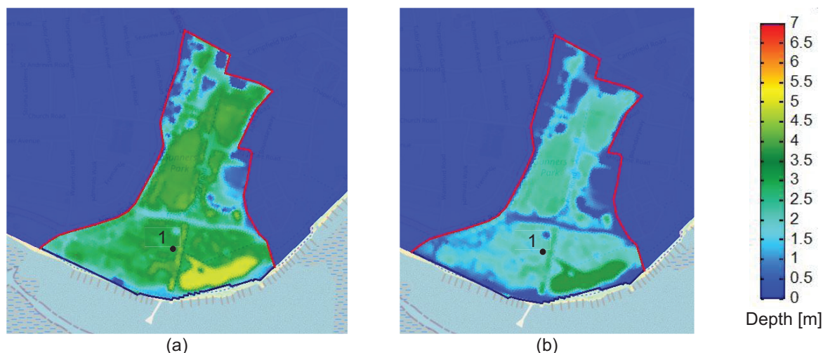
Figure 6. Results of Delft3D FM numerical simulations for the scenarios with additional internal barriers and increased crest heights: (a) crest at 5.2 m; (b) crest at 5.4 m. Both scenarios include SLR of +60cm by 2100.
