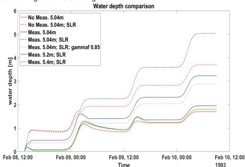
Figure 9. Water depths at location 1 as a function of time for all configurations tested in Sections 3.1 (no measures, current situation), 3.2 (internal protection barriers), 3.3 (Higher coastal protections), 3.4 (Increased roughness).
