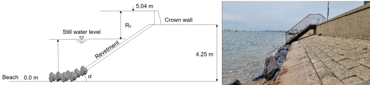
Figure 2. Geometric input of the outer sea wall at Shoeburyness (Southend-On-Sea, UK)
