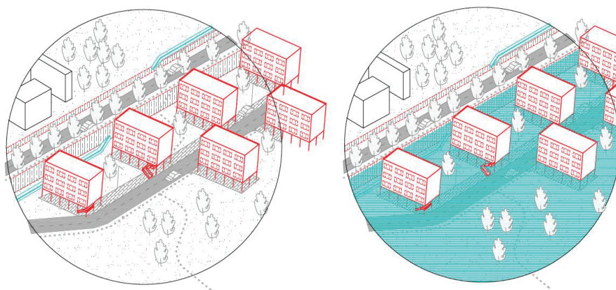
Figure 10. The second line of defence in the background with flood-proof housing developments. [Drawings by A. Bortolotti and L. Iuorio]
