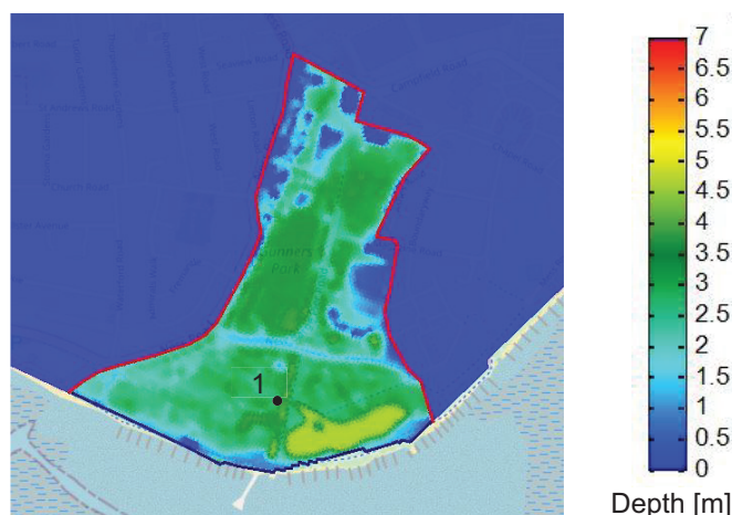
Figure 8. Results of Delft3D FM numerical simulations for the scenario with additional internal barriers and increased roughness on the outer revetment of the dike ( \gamma_f = 0.85 ), including SLR of +60cm by 2100.
