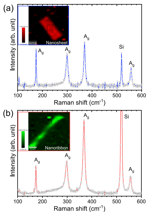
Figure 2. Comparative Raman spectra of TiS 3 (a) nanosheets and (b) nanoribbon measured with 532.5 nm laser line. The inset shows the respective Raman map, which is generated from the A g Raman peak centered at \sim 370 \text{cm}^{-1} .
