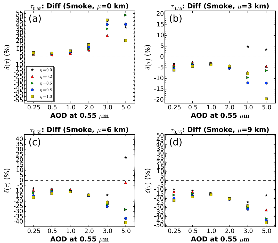
Figure 6. The errors \delta(\tau) of AOD retrievals with different vertical distributions: (a–d) \mu = 0, 3, 6, and 9 km. Smoke model is used in the experiment. The mean differences \delta(\tau) are calculated by averaging over 880 geometrical combinations, shown as a function of aerosol loadings and fine ratios.
