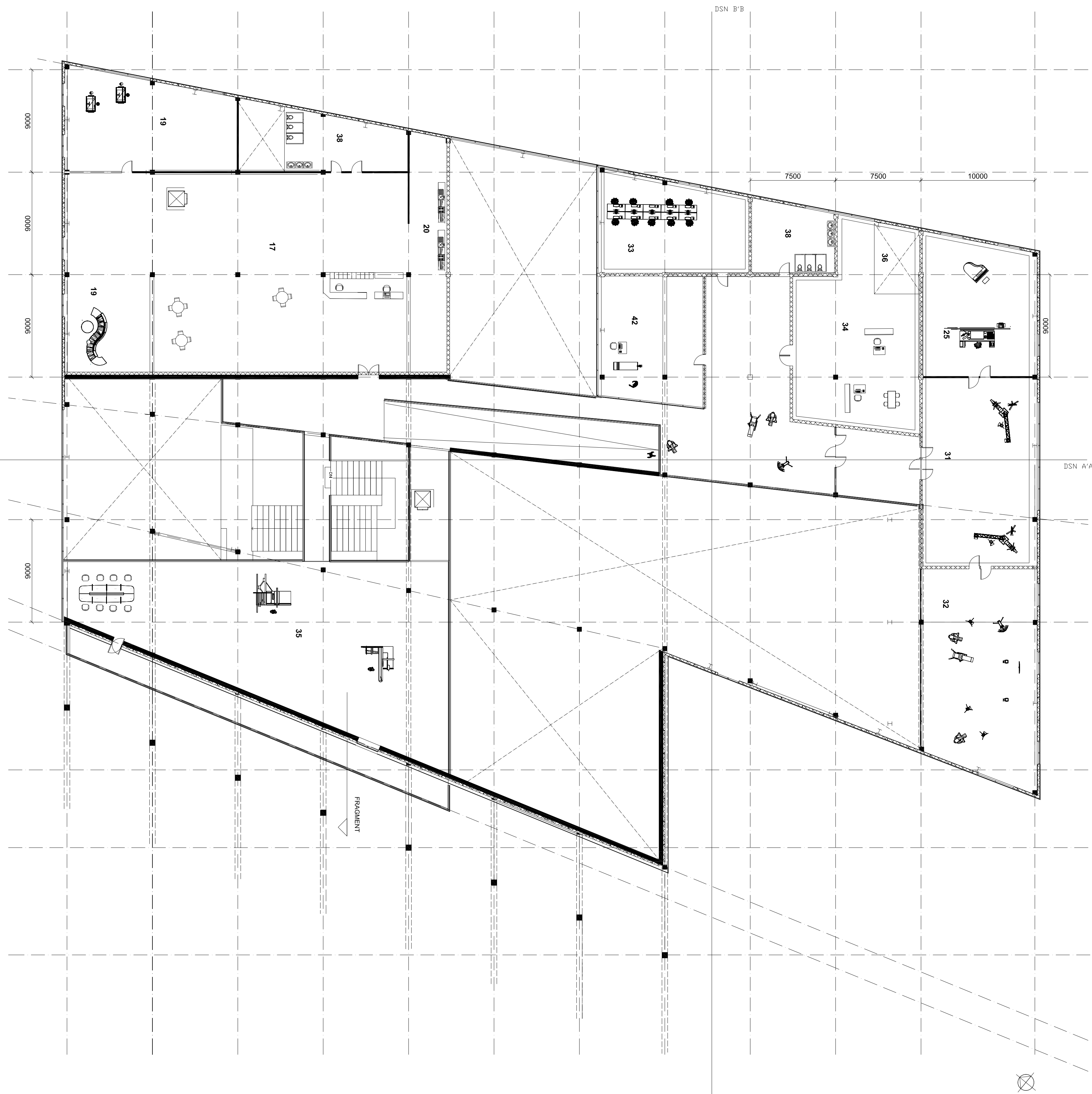
Level 5 1:200
