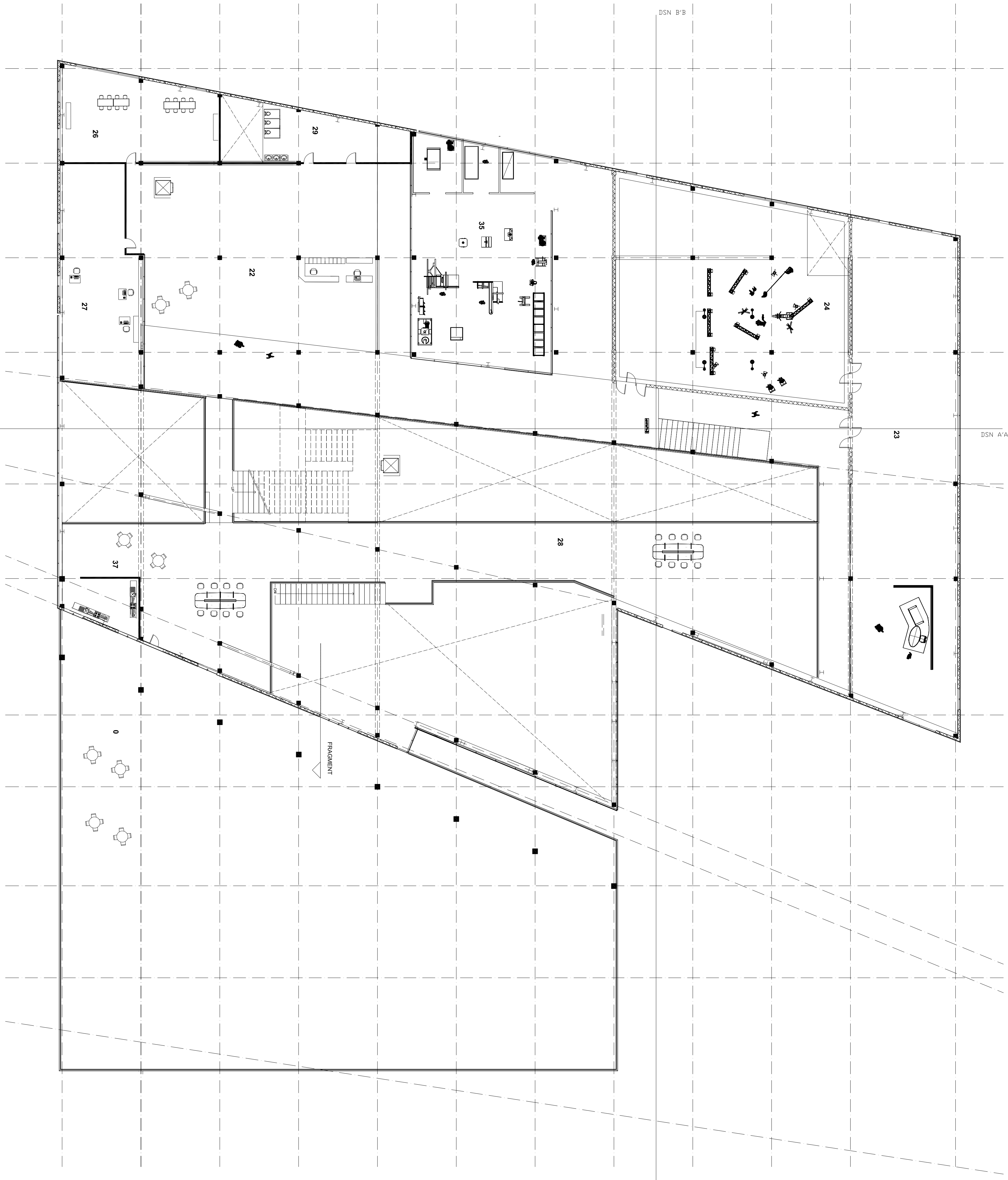
Level 4 1:200
