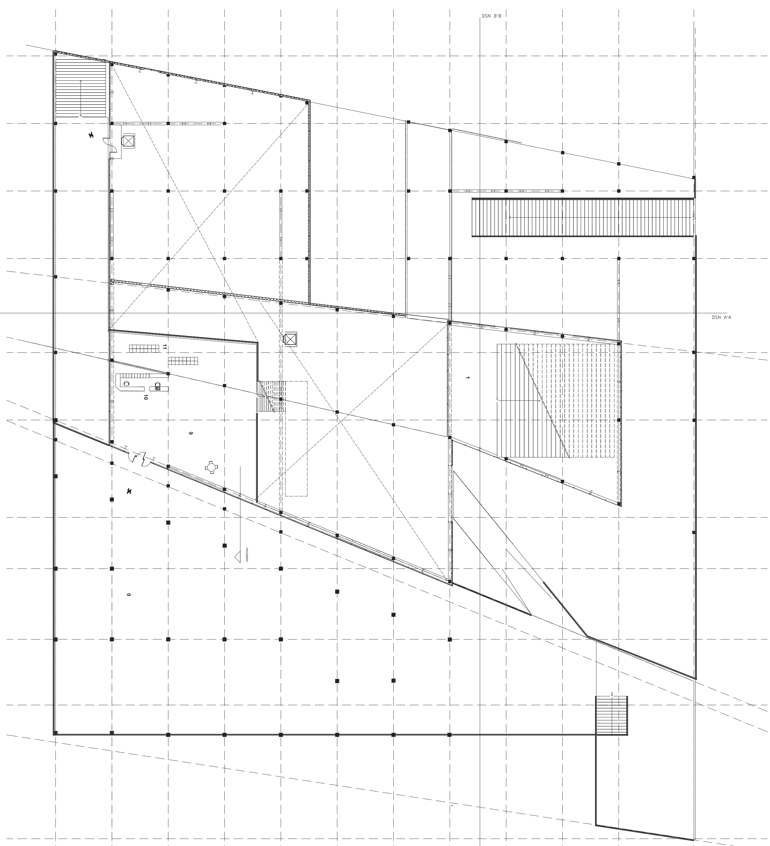
Level 2 1:300
