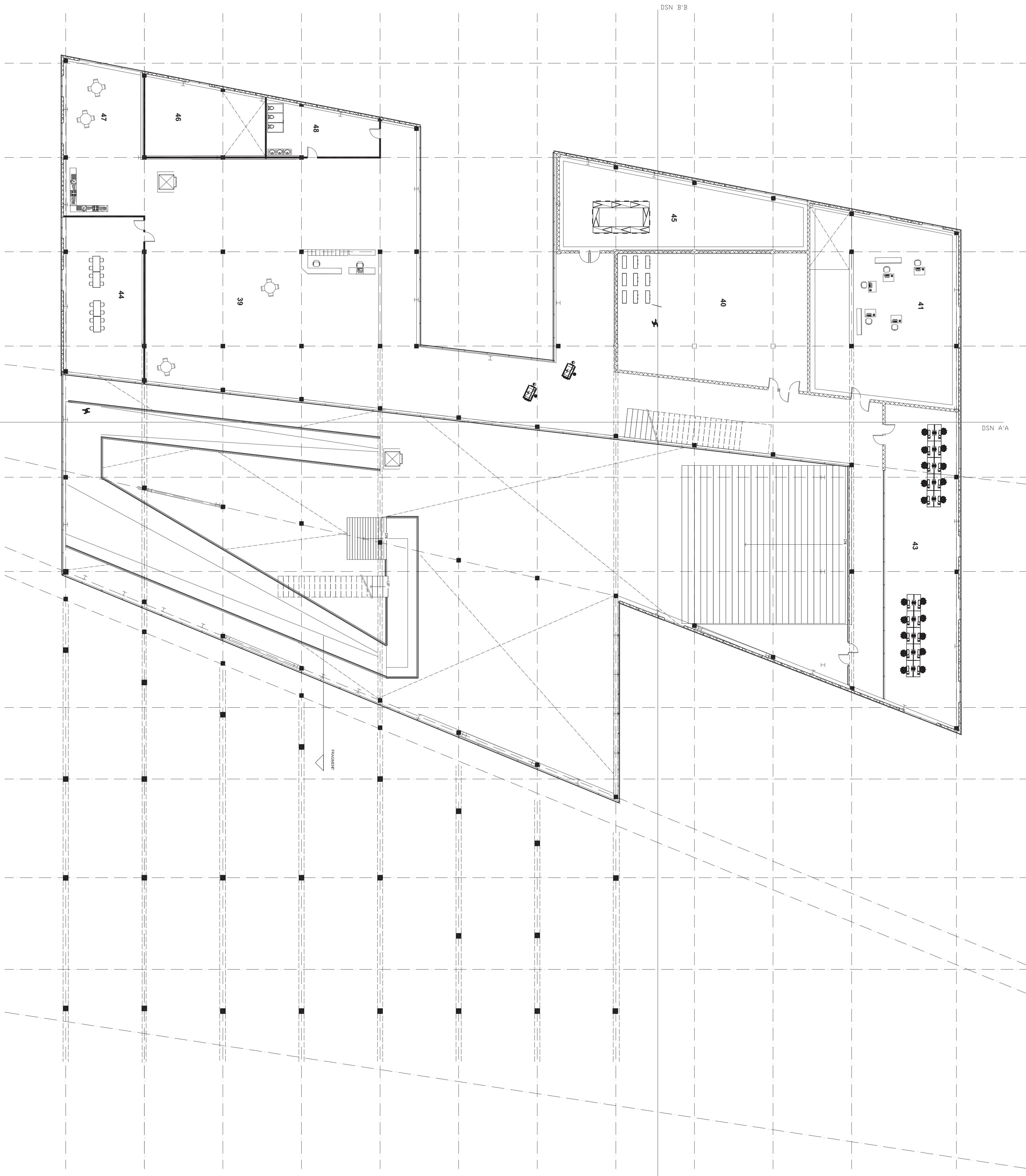
Level 3 1:200
