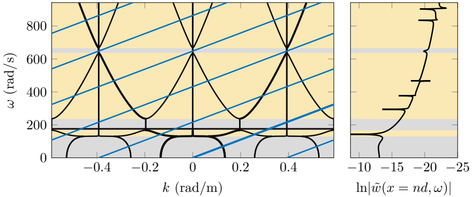
Figure 5.21: The dispersion curves in three Brillouin zones (black lines) and the kinematic invariants (blue lines) (left panel), and the frequency spectrum of the steady-state displacement (right panel); the grey/yellow background represents a stop/pass band.
