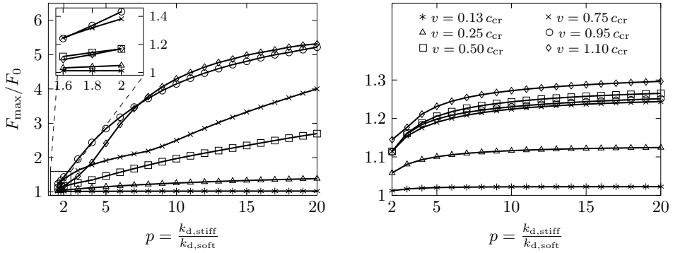
Figure 4.14: Maximum contact force normalized by the dead load versus stiffness ratio for the soft-to-stiff case (left panel) and for the stiff-to-soft case (right panel); l_t = 0.1 m; in the legend, c_{cr} represents c_{cr,l} for the soft-to-stiff case and c_{cr,r} for the stiff-to-soft case.
