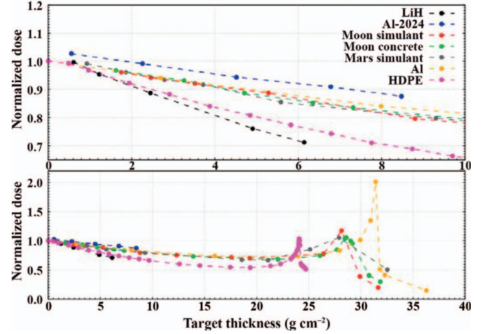
FIG. 2. Partial or full Bragg curves of 968 MeV/u ^{56}\text{Fe} ions in aluminum, high-density polyethylene (HDPE), Moon and Mars simulants and 972 MeV/u ^{56}\text{Fe} ions in aluminum 2024 (Al-2024), lithium hydride (LiH) and Moon concrete. The upper plot shows the datasets magnified up to a depth of 10 \text{ g cm}^{-2} . The characteristics of all materials can be found in Table 1.
