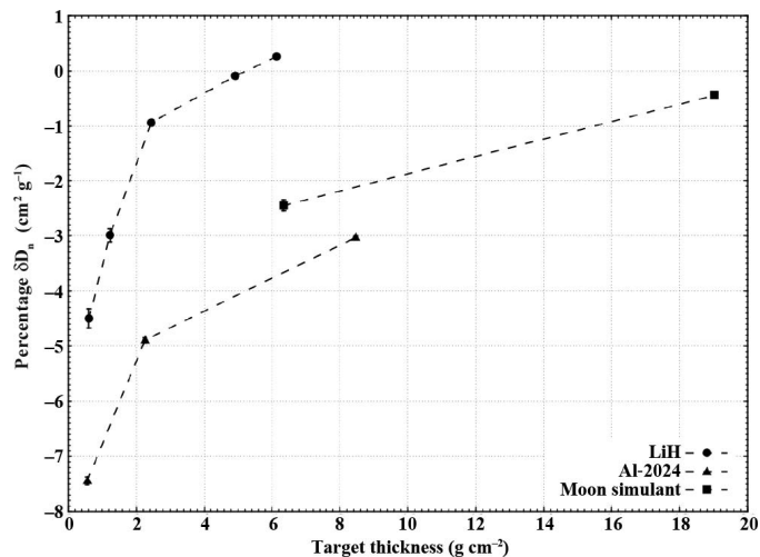
FIG. 8. Normalized dose reduction \delta D_n as a function of depth for several material types exposed to 1,000 MeV/u 4 He ions. The values were calculated using Eq. (2). The characteristics of all materials are shown in Table 1.
