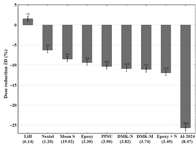
FIG. 9. Dose reduction of single materials exposed to 1,000 MeV/u 4 He ions. The target thicknesses in g cm -2 are reported in parentheses while the exact \delta D values are indicated in percentage on top of each column. The characteristics of all materials are shown in Table 1.
