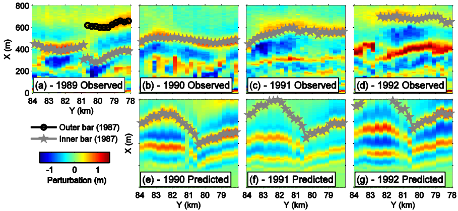
Figure 3.7 Observed (top row) and predicted (bottom row) profile perturbations from 1989 to 1992, black (grey) line tracks the outer (inner) bar starting from 1987.
