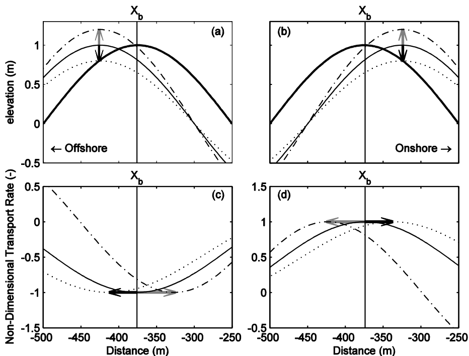
Figure 2.1 Overview of bar response types (a, b) and the initial non-dimensional sediment transport distributions (c, d). Thick solid lines (a, b): initial bar profiles; thin solid lines (a, b): seaward or landward bar migration with constant bar amplitude; dotted lines (a, b): bar amplitude decay during seaward (SD) and landward migration (LD); dash-dotted lines (a, b): bar amplitude growth during seaward (SG) and landward migration (LG). Initial non-dimensional transports (c, d) according to definitions for the bar response types in (a, b). Vertical line indicates the bar crest position, X_b . Arrows (a, b) indicate bar amplitude growth (gray) or decay (black). Arrows (c, d) indicate the associated shift of the transport peaks relative to the initial bar crest position of both types of amplitude response.
