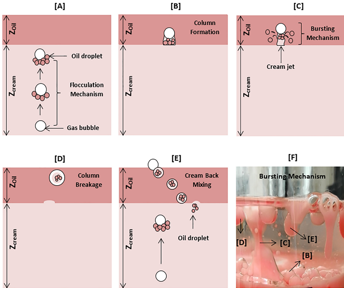
Fig. 2. Schematic representation of the mechanistic model describing oil recovery by GEOR in a cream layer with oil on top: [A] aggregation mechanism – rising of the gas bubble through the cream layer and attachment of oil droplets; [B] Cream jet formation with the oil droplets, previously attached, inside; [C] Rising of gas bubble through the oil layer and oil release due to pressure increase inside the cream jet; [D] Jet breakage and rising of gas bubble with remaining cream and oil; [E] Gas bubble release into the surface and back mixing of cream and oil droplets back to the cream. The cream merges into the cream layer and the oil droplets become available to aggregate to a gas bubble; [F] Experimental picture of the different steps [B–E] when the gas bubbles crosses the interface between the top of the cream layer and the oil layer.
