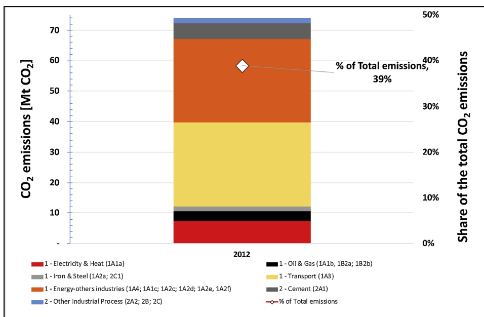
Fig. 1. CO 2 emissions in Colombia from the industrial, energy, and transport sectors (IDEAM et al., 2016). Categories in the legend follow the CO 2 emissions inventory guidelines from (IPCC, 2006). See more data in Appendix 7.1.
