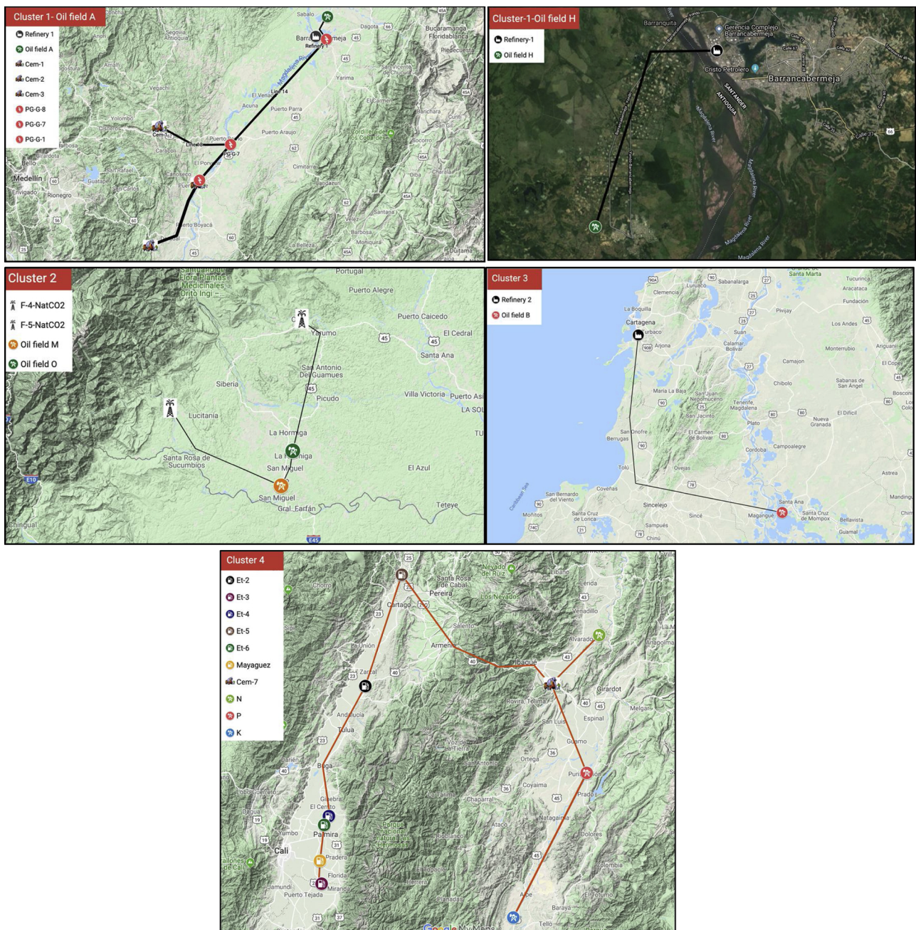
Fig. 9. CO 2 transport infrastructure defined by cluster.
