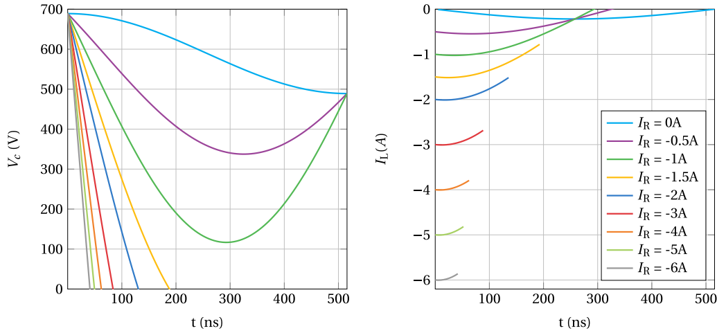
Fig. 7. Voltage across the equivalent capacitance C_{eq} of Fig. 6 and the current through the inductor L_b at that same time in the resonant interval during t_{dead} . ZVS is only achieved when V_c = 0 V. This figure shows that not all values of I_R will lead to ZVS. V_{in} = 689 V, V_o = 100 V, C = 355 pF, L = 75.8 \mu H.
