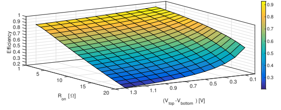
Fig. 3. Power efficiency for different on-resistances with C_{bp} = 5\%C_{fly} . V_{top} = 2.2 V, while V_{bottom} has been swapped from 2.1 V to 0.9 V.
