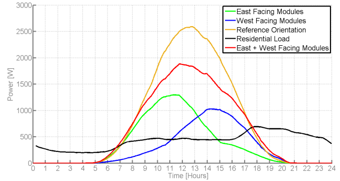
Fig. 12. Power for Optimised Orientation in Autumn
