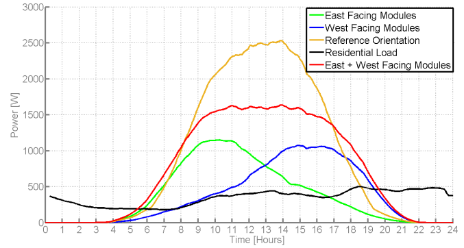
Fig. 11. Power for Optimised Orientation in Summer
