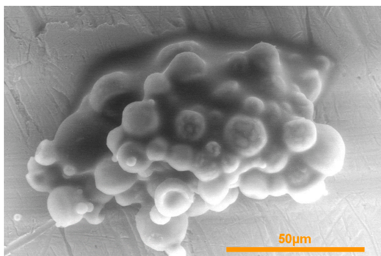
Fig. 10. ESEM image of powder, coated with 5 cycles of SiO 2 , in the presence of moisture.
