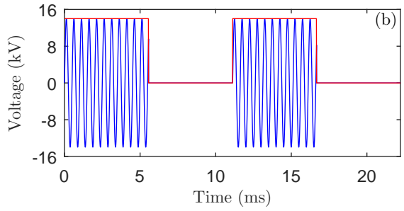
Figure 1: (a) Splitter-plate edge design (not to scale). The aluminium plate (black), the PMMA splitter-plate edge (light gray), the electrodes (red lines) and the epoxy resin encapsulating the grounded electrode (dark gray) is shown. The reference system is also depicted. (b) Sample input waveform (blue) and square-wave burst modulation (red). V_{ac} = 14 kV, f_{ac} = 2 kHz, f_b = 90 Hz.
