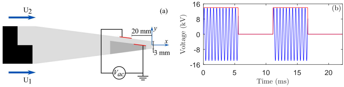
Figure 1: (a) Splitter-plate edge design (not to scale). The aluminium plate (black), the PMMA splitter-plate edge (light gray), the electrodes (red lines) and the epoxy resin encapsulating the grounded electrode (dark gray) is shown. The reference system is also depicted. (b) Sample input waveform (blue) and square-wave burst modulation (red). V_{ac} = 14 kV, f_{ac} = 2 kHz, f_b = 90 Hz.
