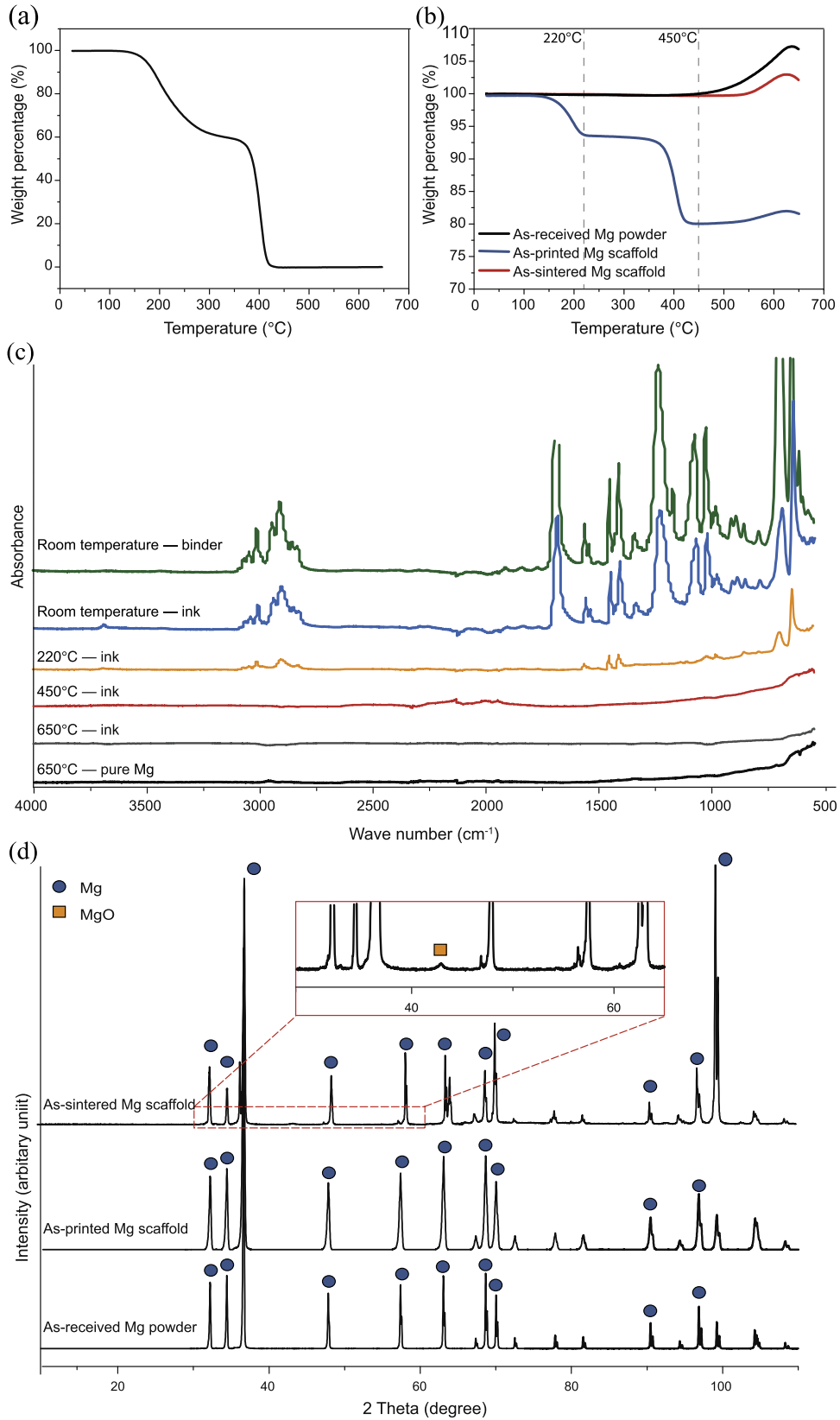
Fig. 6. The characteristics of the decomposition and interaction in the 58 vol% Mg powder loaded scaffold during fabrication process: (a) TGA results of pure binder, (b) TGA results of as-received Mg powders, as-printed and as-sintered scaffolds, (c) FTIR analysis results after the ink was subjected to heating at different temperatures and (d) XRD results of as-received Mg powders, as-printed and as-sintered scaffolds.
