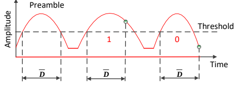
Figure 5.15: Illustration of the PD's captured object-ID signal.
