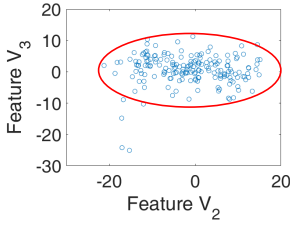
Figure 3.12: Mahalanobis.
