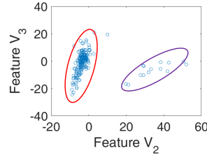
Figure 3.13: Multi-cluster.
