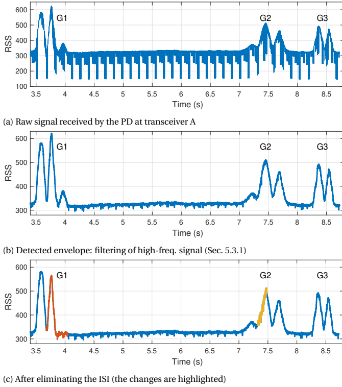
Figure 5.28: Evaluation on passive identification when LEDs operate at the communication+illumination mode.
