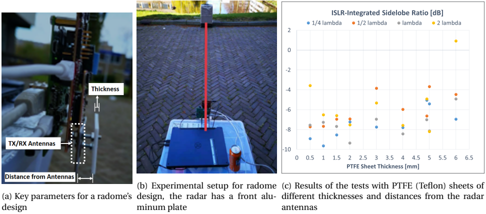
Figure 2.2: The experiments for radome design.
