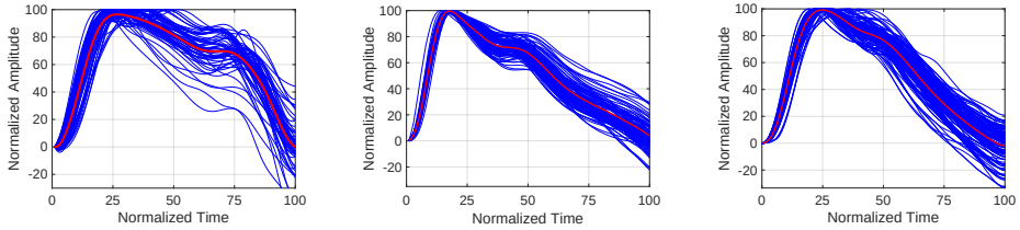
(a) Overlapping periods under default configuration (CTE=4.6735) (b) Overlapping periods under our optimized configuration (CTE=3.4207) (c) Overlapping periods under PPG sensor (CTE=3.4426) Figure 4.7: Comparison of signal stability. The red lines represent the average of all the overlapping periods.
