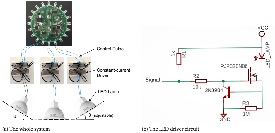
Figure 5.19: Our testbed with the front-end Shine++.
