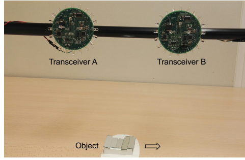
Figure 5.23: Experiment setup in the ideal case (height=15 cm, inter-node distance=20 cm).
