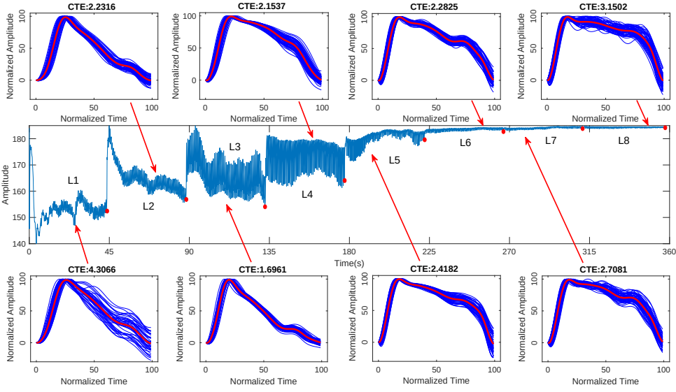
Figure 4.8: Pressure analysis. We apply eight pressure levels on the fingertip of a subject, from 0 N (no pressure) to 21 N (2.1 kg), in steps of 3 N (300 g), in steps of 3 N (300 g). Each pressure level lasts for 45 seconds. Red dots on the PPG signal indicate the end of a pressure level.
