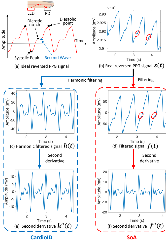
Figure 3.3: Morphology stabilization.
