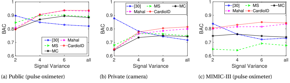
Figure 3.17: Authentication performance.
