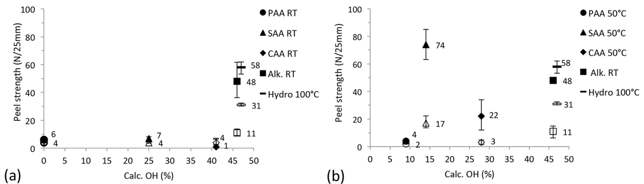
Figure 6: The average dry (empty markers) and wet (filled markers) peel strength vs. the calculated hydroxyl percentage ( \theta = 15^\circ ) on barrier-type oxides for anodizing at RT (a) and 50°C (b) and adhesively bonded with Redux 775 phenolic adhesive (no primer). The error markers represent the minimum and maximum measured values.
