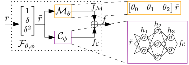
Fig. 2: Feedforward filter \mathcal{F}_{\theta, \phi} with model \mathcal{M}_\theta and neural network \mathcal{C}_\phi , here with N_\theta = 3 and L = 3 hidden layers.
