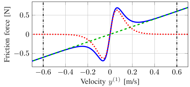
Fig. 3: Stribeck-like friction curve of example system (30) with c_1 = 1 , c_2 = 20 , \alpha = 20 . The nonlinearity g_y ( \cdots ) is approximately zero outside \mathbb{X} ( - - ). The full friction curve ( \text{—} ) approximately coincides with the linear viscous damping ( - - ) for high velocities.
