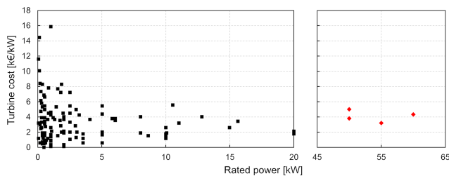
Figure 5. Turbine purchase cost survey for rated power lower than 20 kW (Kaldellis and Zafirakis, 2012) and around 50 kW (authors’ experience).
