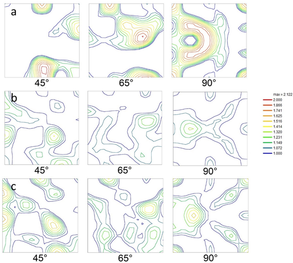
Figure 6. ODFs of retained austenite plotted at the \phi = 45^\circ , 65^\circ and 90^\circ of the Q & P steel prior to testing (a) and after being strained in a static tensile experiment till uniform strain (US) at room temperature (RT) (b) and at 80^\circ\text{C} (c).
