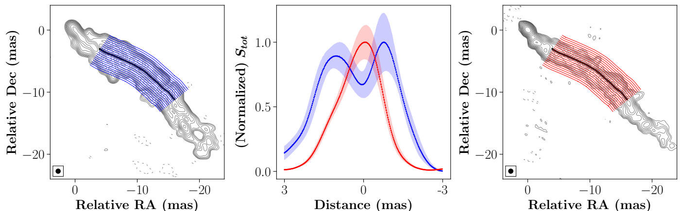
Fig. 5. The 300 jet streamlines used to calculate the integrated flux density along the flow, parallel to the jet axis from MOJAVE (central line in black), overplotted on the 1.6 GHz (left panel) and 4.8 GHz (right panel) RadioAstron contours maps (both convolved with the MOJAVE beam). The starting point is set at 4 mas from the core, where the spine/sheath structure becomes evident. Central panel: integrated flux density, versus distance from jet axis, calculated along jet streamlines for the 1.6 GHz (left) and 4.8 GHz (right) RadioAstron images. The profile uncertainty is reported as a shaded area.
