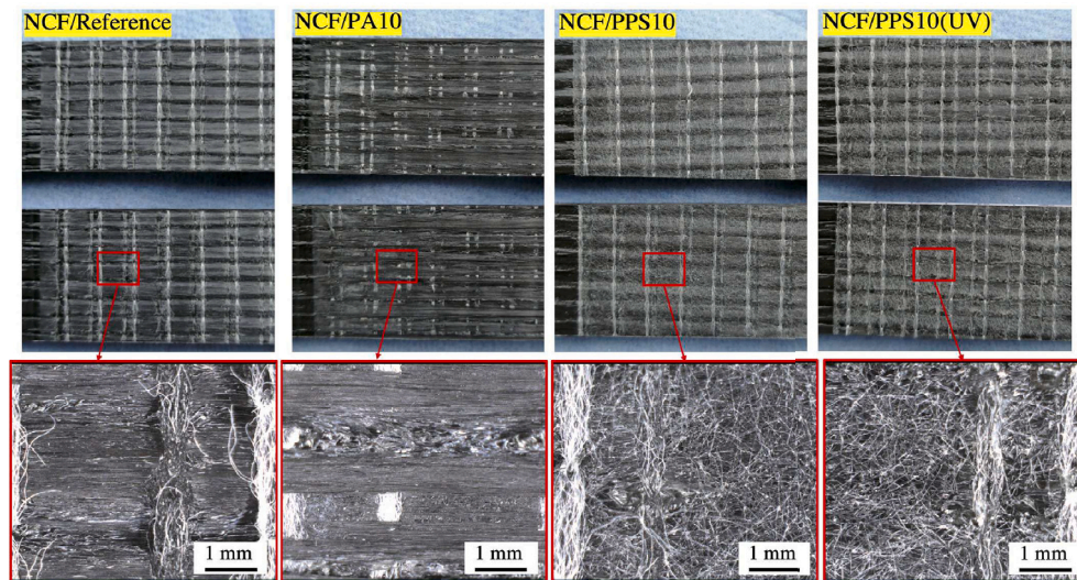
(a) Photos of the fracture surface
