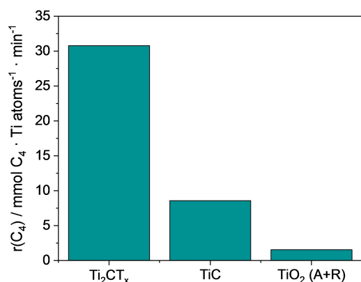
Figure 2. C_4 olefin formation rate of the studied catalysts after 0.5 h under reaction at 500 °C and O_2/\text{butane} = 1:1 . A + R denotes anatase + rutile titania.
