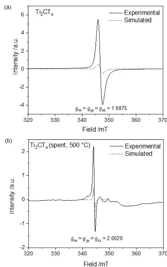
Figure 3. Experimental (measured at 10 K) and simulated EPR spectra of (a) Ti_2CT_x MXene fresh and (b) after the stability test at 500 °C. Experimental parameters; microwave frequency (a) 9.648388 GHz and (b) 9.647805, power 0.6325 mW, modulation amplitude 4.000 G.
