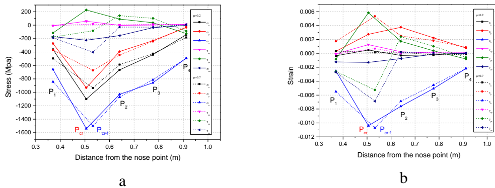
Figure 17. Results of friction coefficients variation: stress and strain components at five selected elements: (a) stress components, (b) strain components
