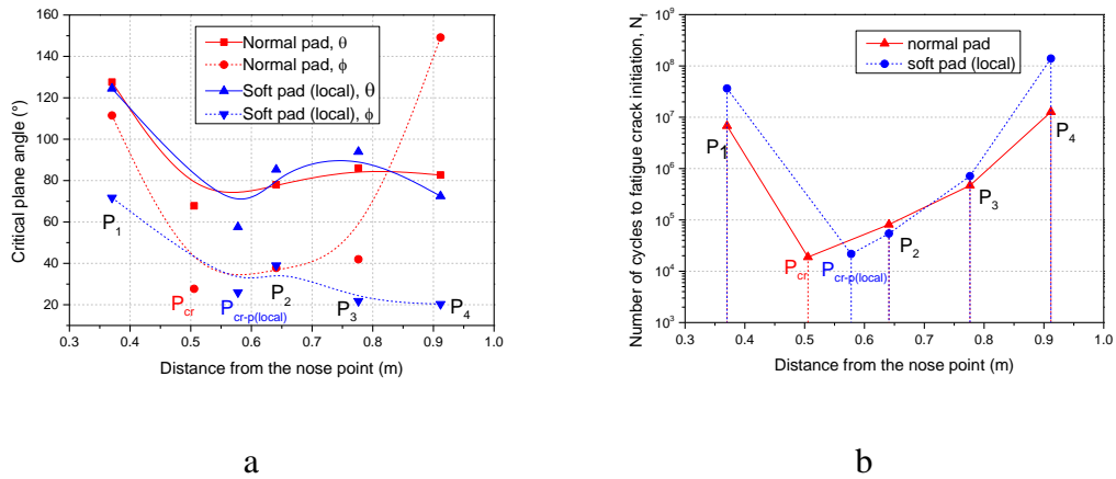
Figure 16. Results of railpads stiffness variation (v01 and v03): fatigue life prediction of: (a) angles of the critical planes, (b) number of cycles to fatigue crack initiation
