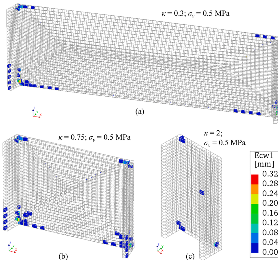
Fig. 14. The tensile failure of the bricks in cases: (a) \kappa = 0.3 , \sigma_v = 0.5 \text{ MPa} ; (b) \kappa = 0.75 , \sigma_v = 0.5 \text{ MPa} ; (c) \kappa = 2.0 , \sigma_v = 0.5 \text{ MPa} . Ecw1 is the principle crack width.
