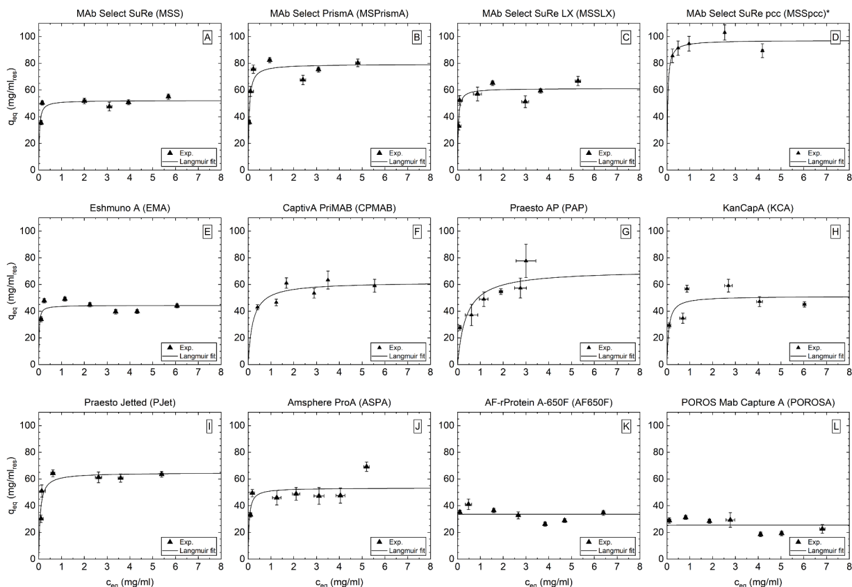
Fig. 2. Adsorption isotherms of mAb on different Protein A resins, in 1x PBS buffer, pH 7.14. Solid lines represent the fit of the experimental data to the Langmuir isotherm. A – MSS; B – MSPrismA; C – MSSLX; D – MSSpcc; E – EMA; F – CPMAB; G – PAP; H – KCA; I – PJet; J – ASPA; K – AF650F; L – POROSA.
