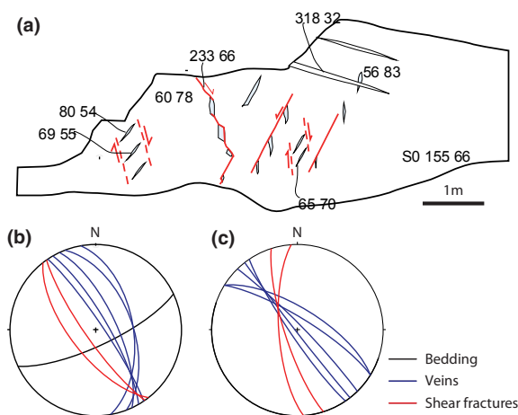
Fig. 12. Syn-subsidence deformation in the Upper Cretaceous Berda Formation (Central Tunisia); (a) Line drawing and stereonet of outcrop TU4 (Selja gorge, Alima anticline). The surface shown in the drawing corresponds the lower bedding surface of a steeply SE dipping layer. The gently dipping veins visible in the upper part of the outcrop are associated with folding and not considered here. (b) stereonet of the geometric elements shown in the line drawing; (c) geometric elements position of fractures and veins once bedding is rotated back to horizontal.
